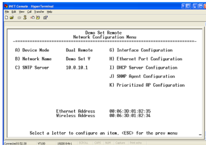
Figure 2-14. Network Configuration Menu From Remote Unit
