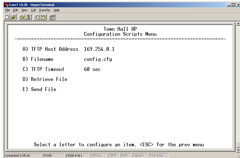
Figure 2-66. Configuration Scripts Menu
