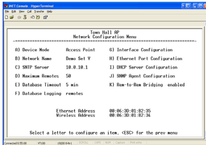
Figure 2-13. Network Configuration Menu From Access Point
