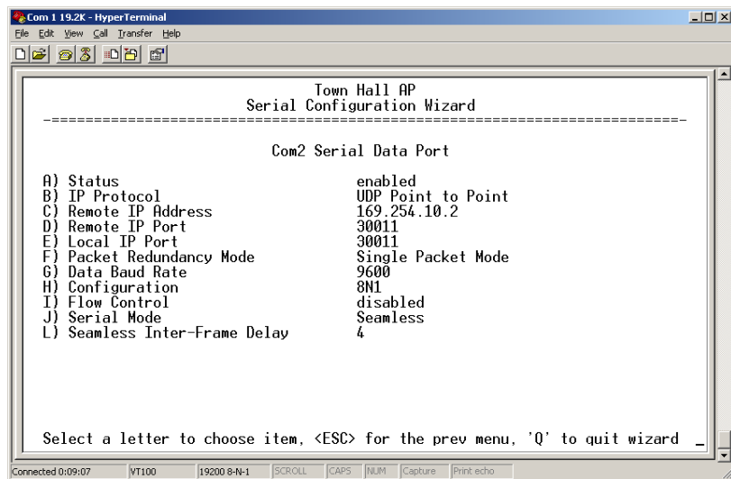
Figure 2-32. UDP Point-to-Point Menu
