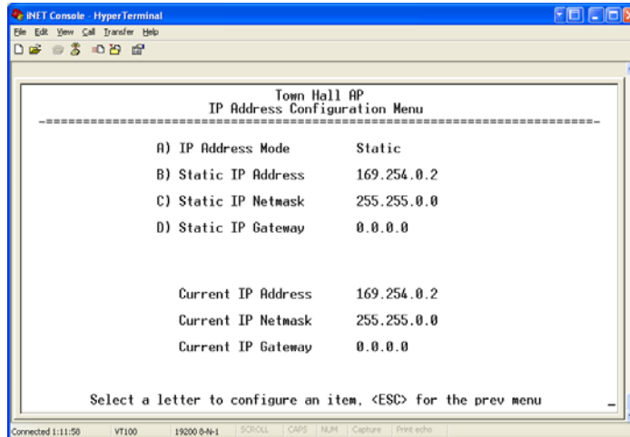
Figure 2-19. IP Address Configuration Menu
