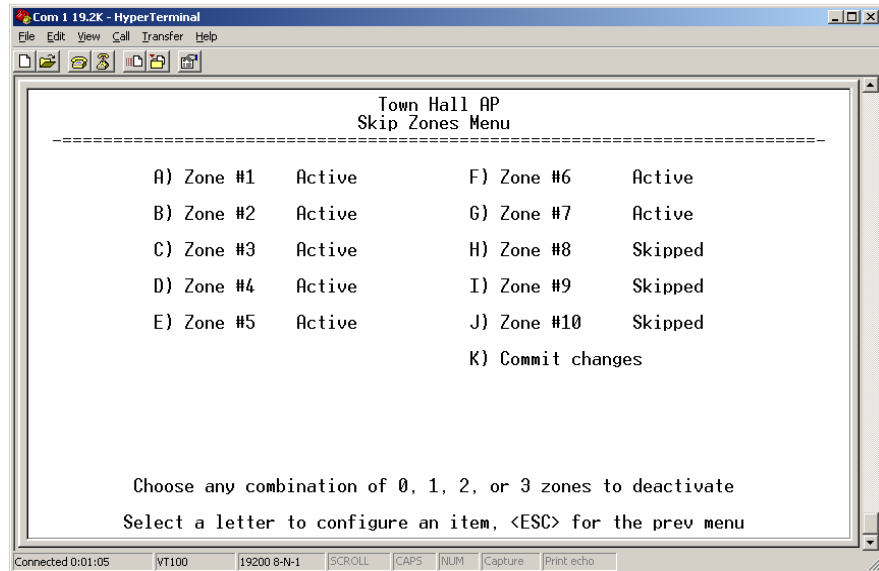
Figure 2-27. Skip Zone Options Submenu—GE MDS iNET Only (“Commit changes” displayed only on Access Point radios)
