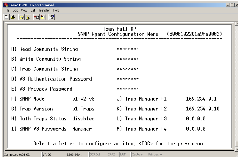
Figure 2-22. SNMP Server Configuration Menu From Access Point
