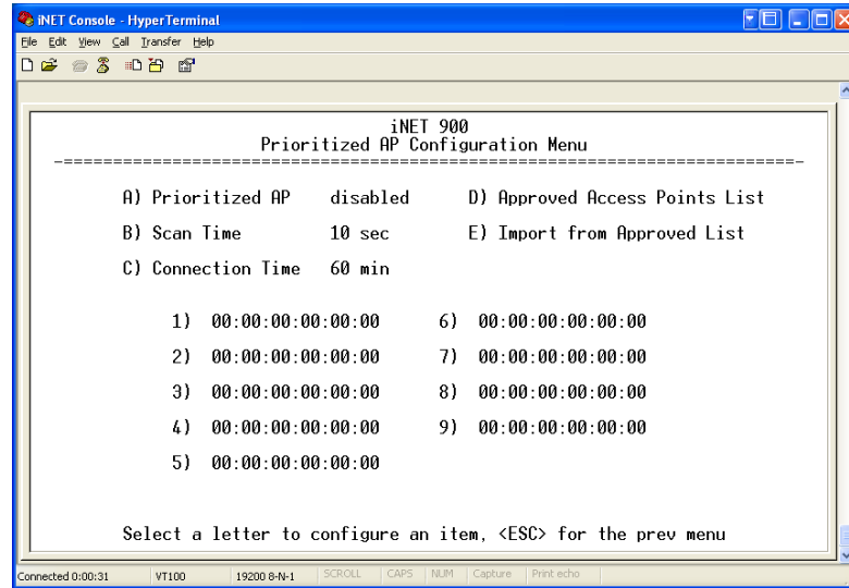
Figure 2-23. Prioritized AP Configuration Submenu
