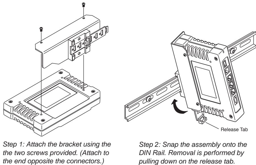
Figure 4-4. DIN Rail Mounting of GE MDS Equipment
