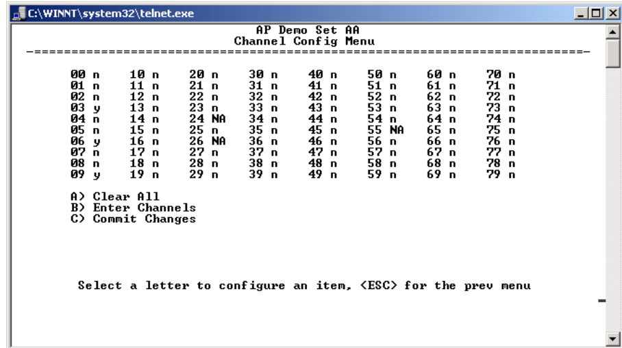
Figure 2-26. Channel Config Submenu
