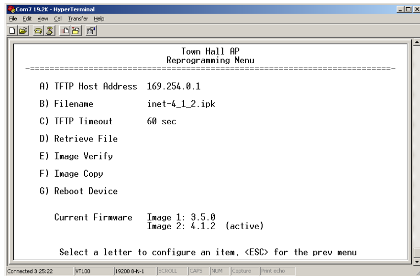
Figure 2-63. Reprogramming Menu (Shown with "Image Copy" Selected)
