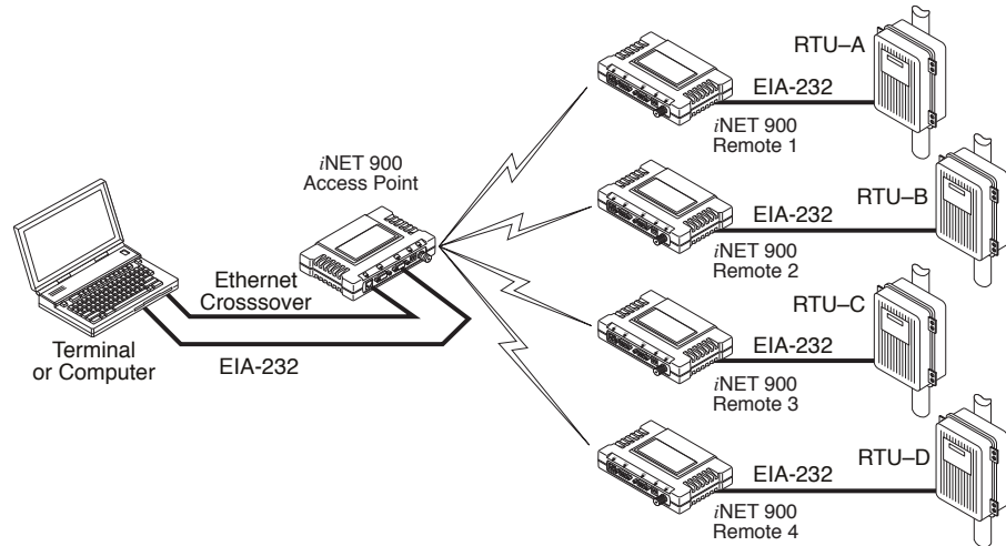
Figure 2-40. Mixed-Modes Application Diagram
