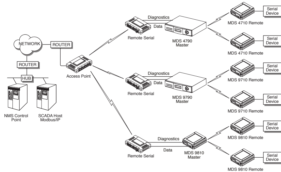
Figure 1-5. Backhaul Network
