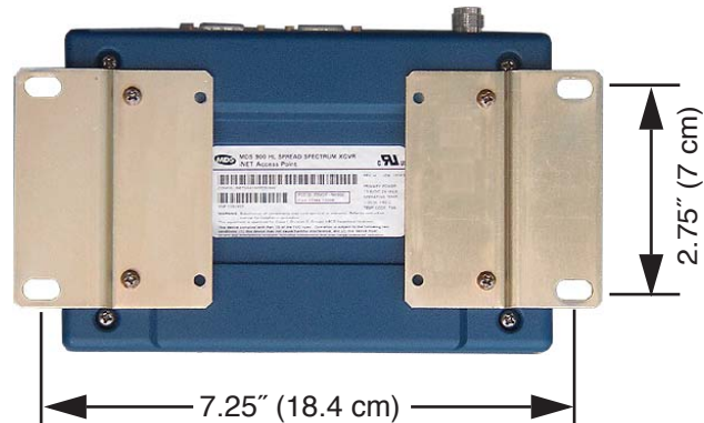
Figure 4-3. Mounting Bracket Dimensions
