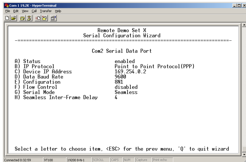
Figure 2-35. PPP Menu
