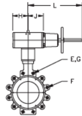
Double Acting Sizes 210 thru 280
