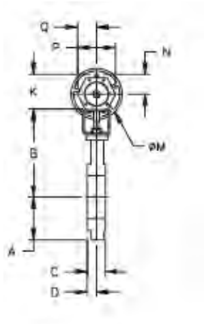
Double Acting Sizes 210 thru 280
