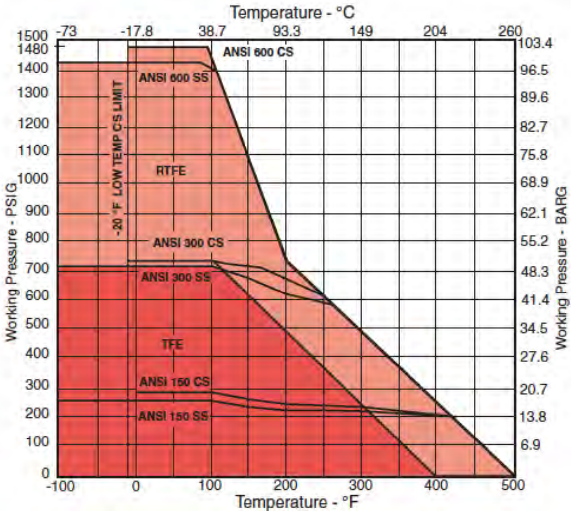
ANSI B16.34 Body and Flowseal Soft Seal Pressure - Temperature Ratings
