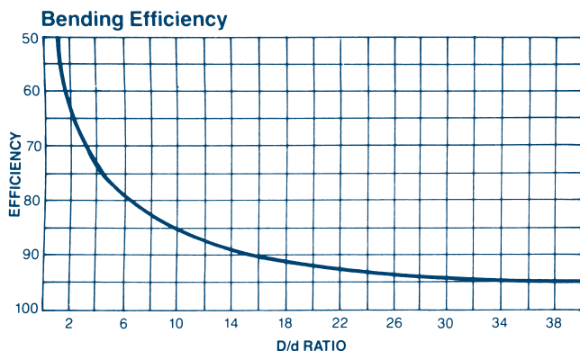
Efficiency falls as the D/d ratio becomes smaller. This curve, based on static test data only, illustrates the decline of bending efficiency for 6 x 19 and 6 x 37 classification ropes as the D/d ratio is reduced.
