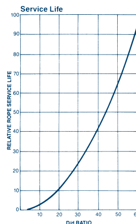
Service life increases as the D/d ratio becomes larger. This curve, based on bending and tensile stresses only, illustrates the relative performance increase.
