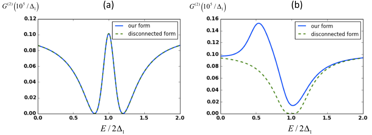
FIG. 2. The two-photon correlation function G^{(2)}(\tau = 10^5 / \Delta_1) as a function of the two photons' total energy E when k_1 = k_2 = E/2 and \gamma_1 = \gamma_2 = \Delta_1/5 . In both cases, the initial and final states of the atom are the ground state |g_1\rangle . (a) \Delta_2 = \Delta_1 . In this case, our result (A13) is the same as the commonly anticipated disconnected form and thus the two-photon correlation functions are identical. (b) \Delta_2 = \Delta_1/2 . In this case, our main result (A13) leads to a significant “bump” in the two-photon correlation function as compared with the disconnected form.
