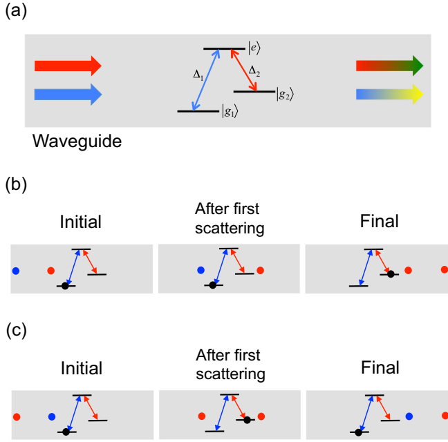
FIG. 1. (a) The system we consider: a photonic waveguide coupled to a three-level \Lambda -type atom. (b) A sequential scattering event where two photons incident from the left scatter against a three-level atom with \gamma_1 = \gamma_2 \ll \Delta_1, \Delta_2 . The photons are represented by red or blue colors with different colors representing different frequencies of photons. We send in the red photon followed by the blue photon, in which the initial, intermediate, and final states are shown in the subplots. (c) Another sequential scattering event that is the same as in panel (b) except for the reverse photon ordering.
