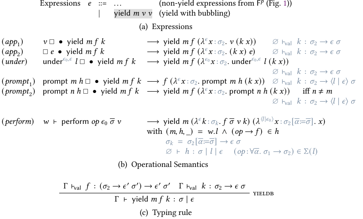
Fig. 10. F^{pb} : Multi-prompt with bubble semantics.
