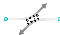
At low speeds, electromagnetic repulsion prevents the collision of nuclei
