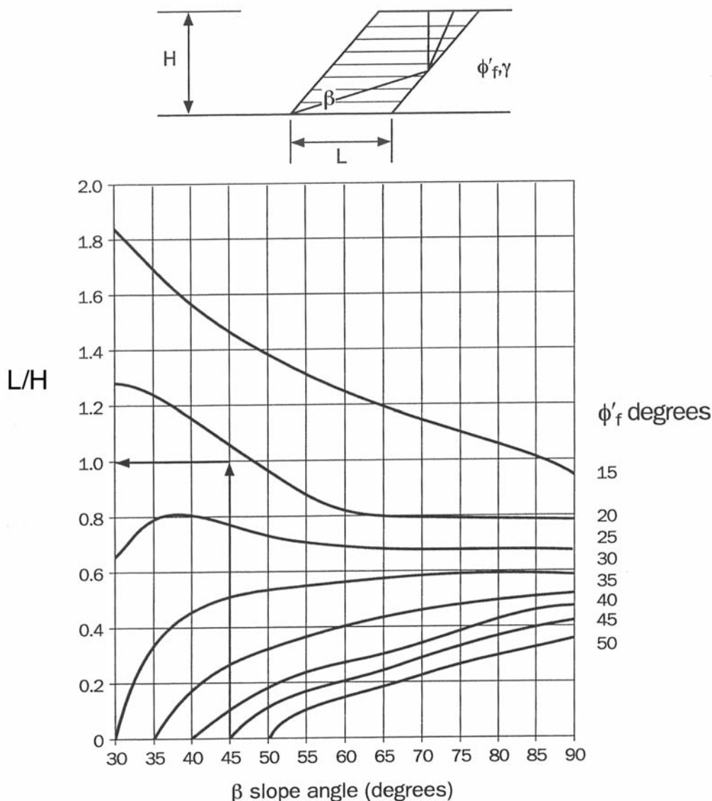
Chart 2: Minimum Ratio of Reinforcement Length to Slope Height L/H to contain Critical Two-Part Wedge and Satisfy Sliding and Eccentricity Criteria.
