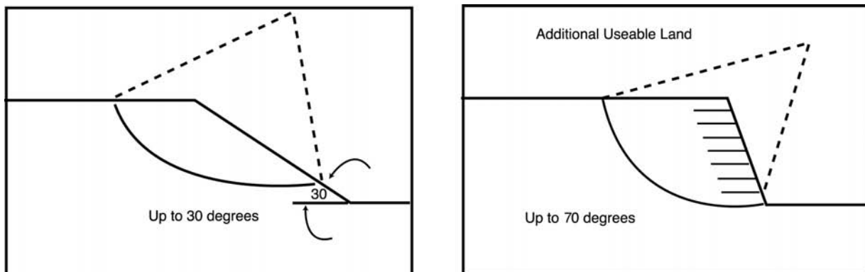
Figure 2: Conventional vs. Steepened Slopes
