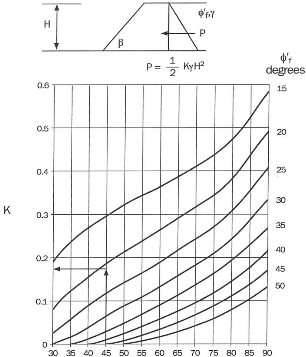
Chart 1: Equivalent Coefficient of Earth Pressure, K = f(\phi'_f, \beta)
