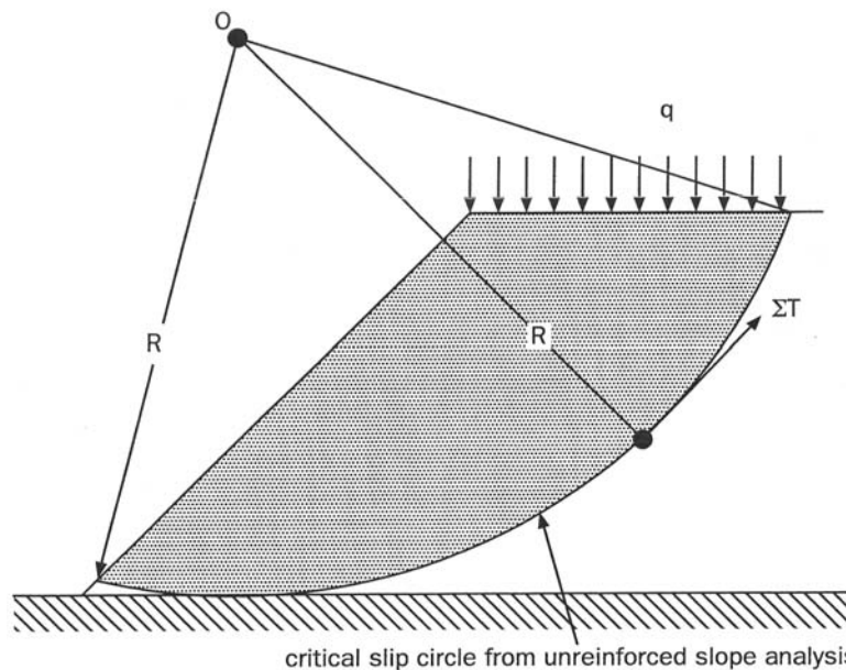
Figure 8: Approximate Method to Calculate the Factor-of-Safety for a Reinforced Slope (3)
