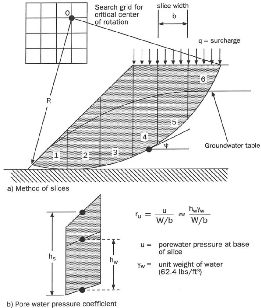
Figure 6: Circular Slip Analysis and Method of Slices for Unreinforced Slope
