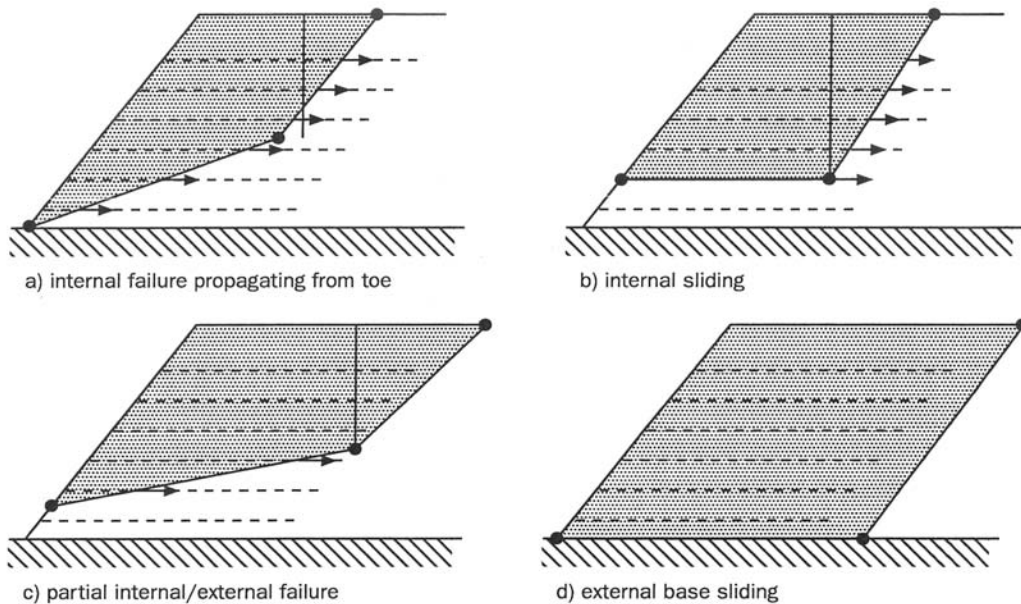
Figure 5: Some Two-Part Wedge Failure Mechanisms
