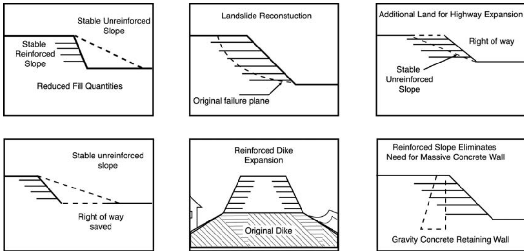
Figure 1: Applications Using Reinforced Steepened Slopes
