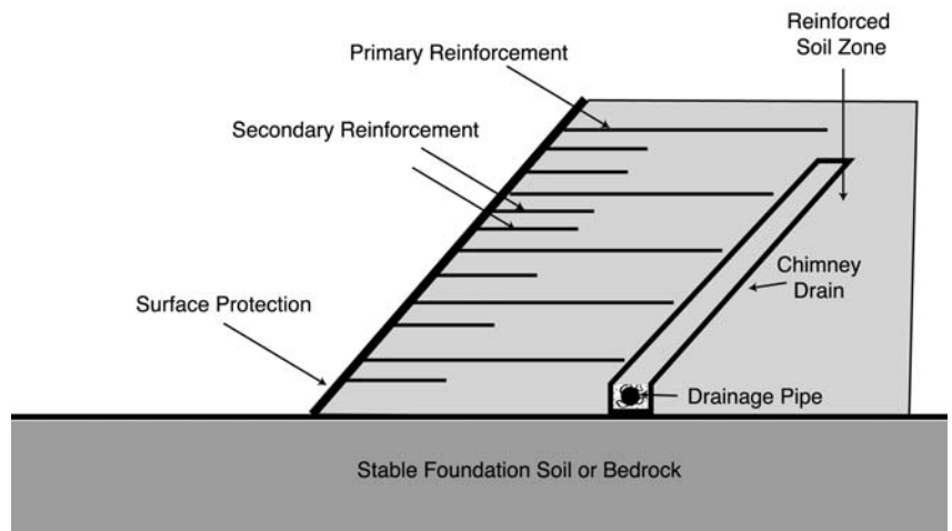
Figure 3: Typical Components of a Reinforced Steepened Slope System
