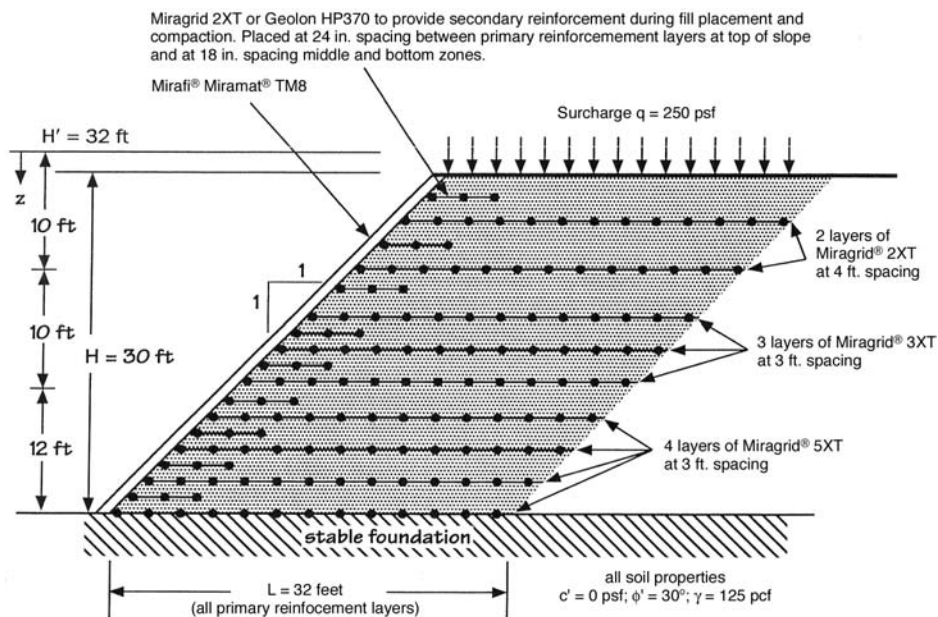
Example Figure 3: Example Miragrid® Reinforcement Layout
