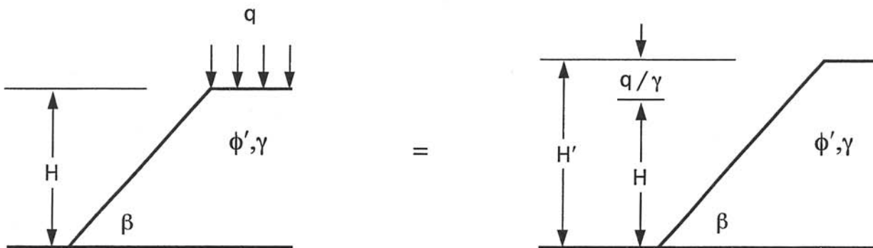
Figure 13: Modified Slope Height to Incline Influence of Uniformly Distributed Surcharge
