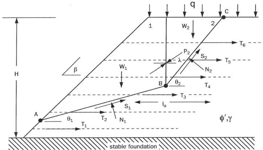
Figure 4: Two-part wedge analysis
