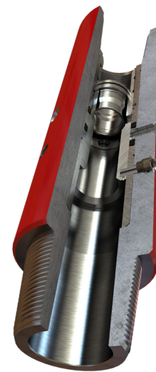
Top Down Squeeze Valve
