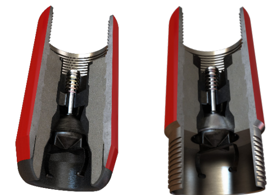
Float Shoe
