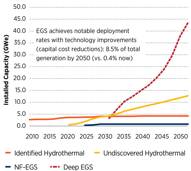
Figure 4-3. Technology Improvement scenario results by resource type
