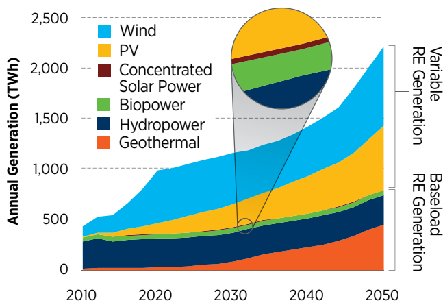
Figure 4-4. Total national generation (terawatt-hours) for the renewable energy (RE) market sector by year for the GeoVision Technology Improvement scenario
