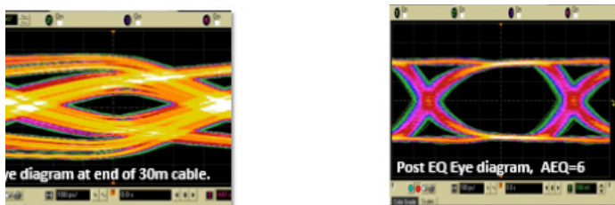
Figure 9. Contrast Between Closed (left) and Open (right) Eye Diagrams
