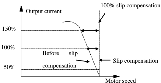
Fig.6-13 slip freq. compensation
