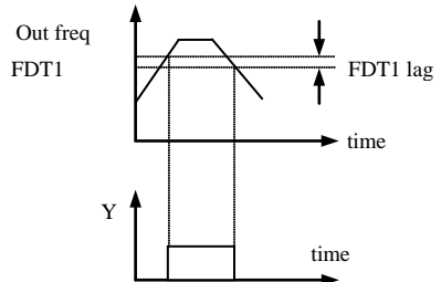
Fig. 6-27 freq level detection
