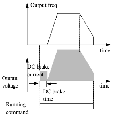
Fig.6-11 start mode 1
