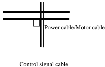
Fig. 3-16 Orthogonal wiring
