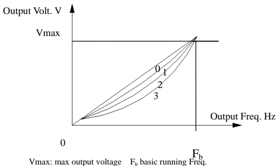
Fig. 6-7 V/F curve
