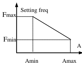
(2) Negative effect
