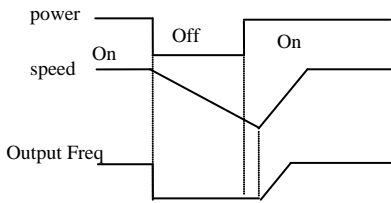
Fig.6-9 Speed tracking restart
