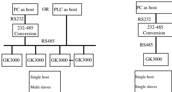
Fig. 9-1 Networking of slaves
