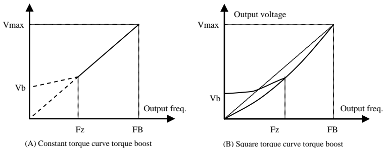
Fig.6-3 Torque boost
