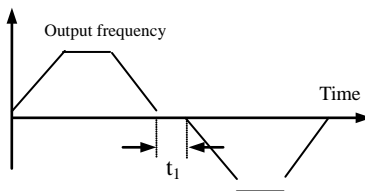
Fig.6-1 FWD/REV dead
