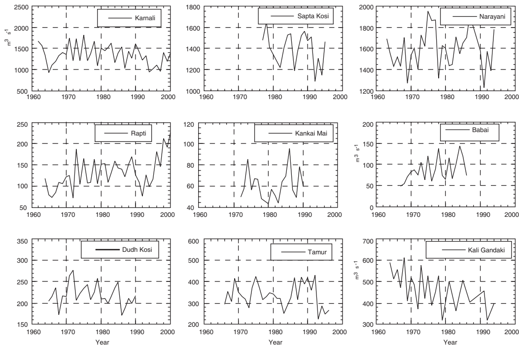
FIGURE 15: Discharge data of selected rivers: Large rivers (top); Southern rivers (middle) and Snowfed rivers (bottom)
