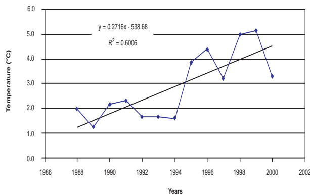
FIGURE 13: Annual mean temperature trend in Kyangjing, Langtang station (3,900 m).
