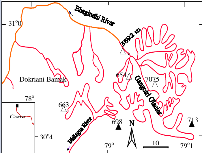
FIGURE 23: Drainage map of the Bagirathi River, Garhwal Himalayas
