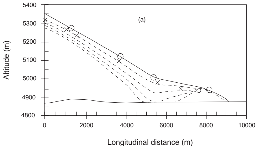
FIGURE 10: The longitudinal profile of Khumbu Glacier. The solid line represents profile of 1978, the dashed line represents simulated result for 1999 and dotted lines are simulated results for 2020, 2040 and 2060. The circles and cross symbols represent survey positions in 1978 and 1999 respectively.
