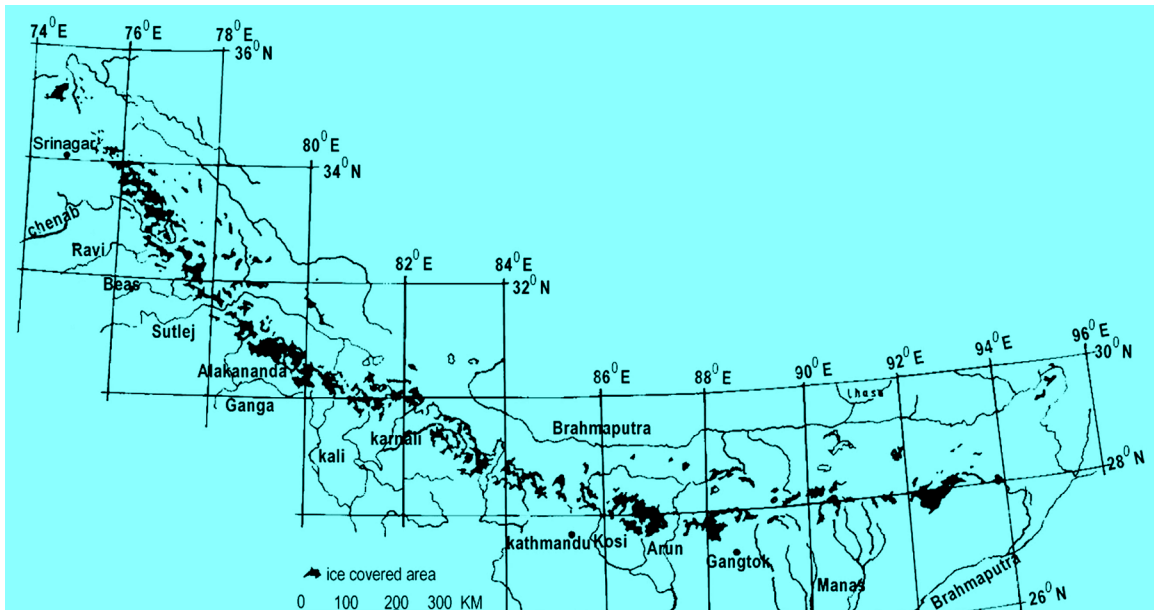
FIGURE 19: Glacier distribution along the Himalayan arc
