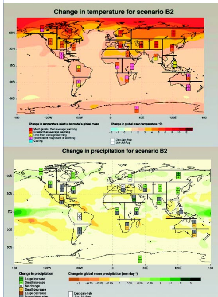
FIGURE 7: Changes in temperature (top) and precipitation (bottom) for SERES scenario B2. The background shows the annual mean changes and the boxes shows inter-model consistency in regional temperature and precipitation changes.
