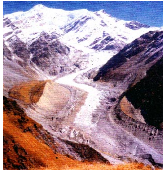
FIGURE 22: Synoptic view of the Dokriani glacier
