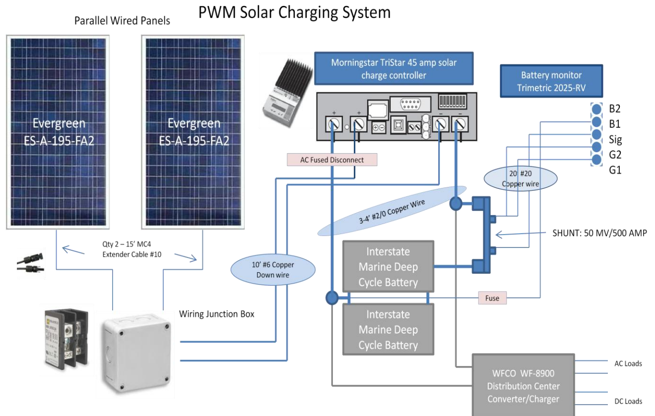
FunFinder Solar System Block Diagram
