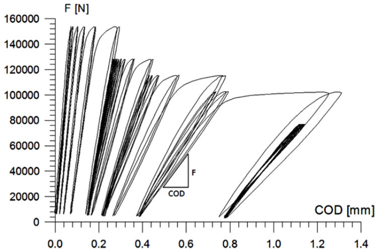
Figure 3. Relationship of F - COD recorded in subsequent overload cycles of fatigue crack growth test
