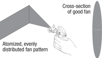
Low pressure spray with air "assisting" the spray pattern
