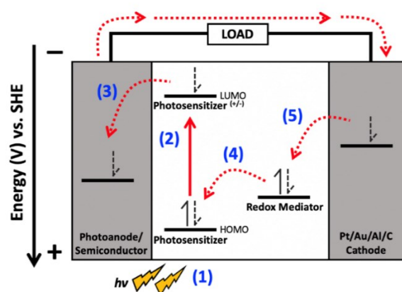
Figure 2. Representation of electron transfer in a photovoltaic device. This is comprised of a photosensitive dye(s), semiconductors, and electrolyte (redox mediator). In order for forward electron
