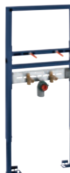
39 052 000 Rapid SL for wash basin height adjustable, for single hole installation, 1.13 m installation height, for on-the-wall installations or studded walls, 2 noise protected fitting connections 1/2"
