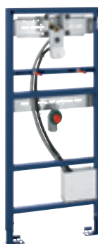
38 748 001 Rapid SL for wash basin with roughing-in set for infra-red electronics Allure E, Essence E and Europlus E for installation with pre-mixed or cold water 1.13 m installation height
