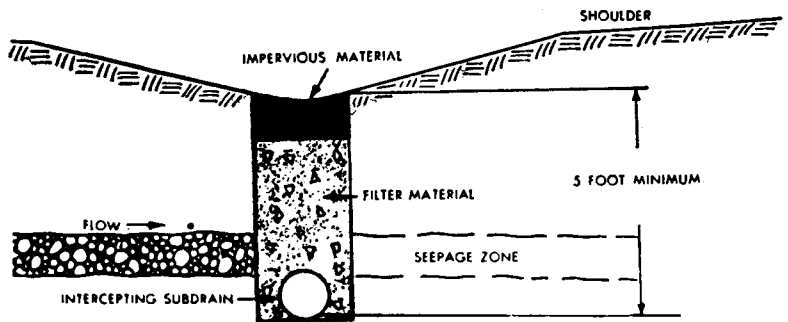
Figure 4.—Intercepting subdrain for a roadway (Aviation Engineers, War Dept. Tech. Manual 5-255, fig. 49, p. 125, 1944. Reproduced by permission of the Dept. of the Army.)
