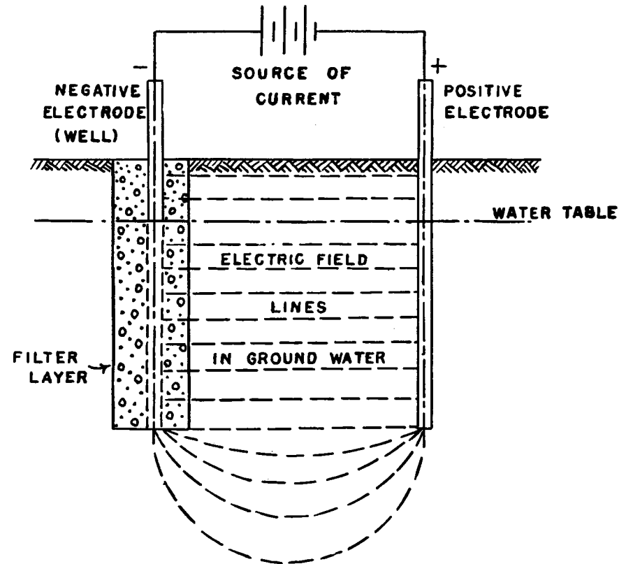
Figure 8.—Schematic diagram of a drainage well, supplied with water by electroosmosis.
