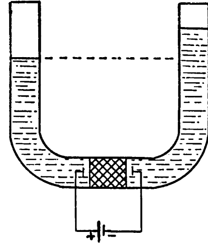
Figure 7.—Electroosmosis through a clay diaphragm in a U-tube. (Adapted from Vey, 1948.)
