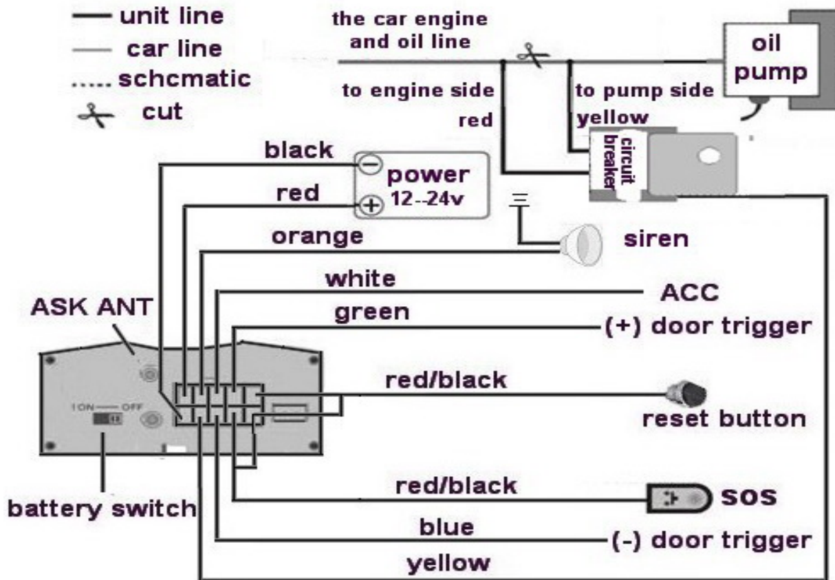
Wiring diagram
