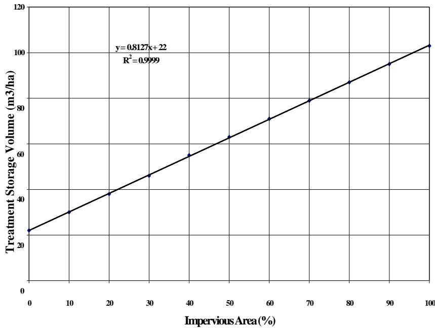
Figure 2.2 Wetland Treatment Storage Volumes
