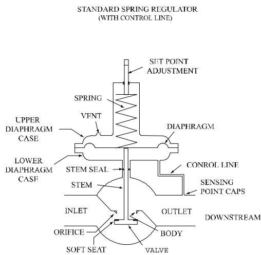
Figure II-4C Single Port Spring Regulator
