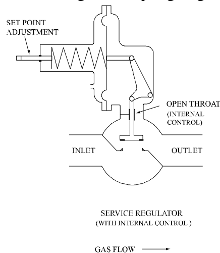
Figure II-4C Single Port Spring Regulator
