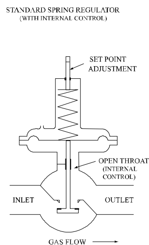
Figure II-4C Single Port Spring Regulator
