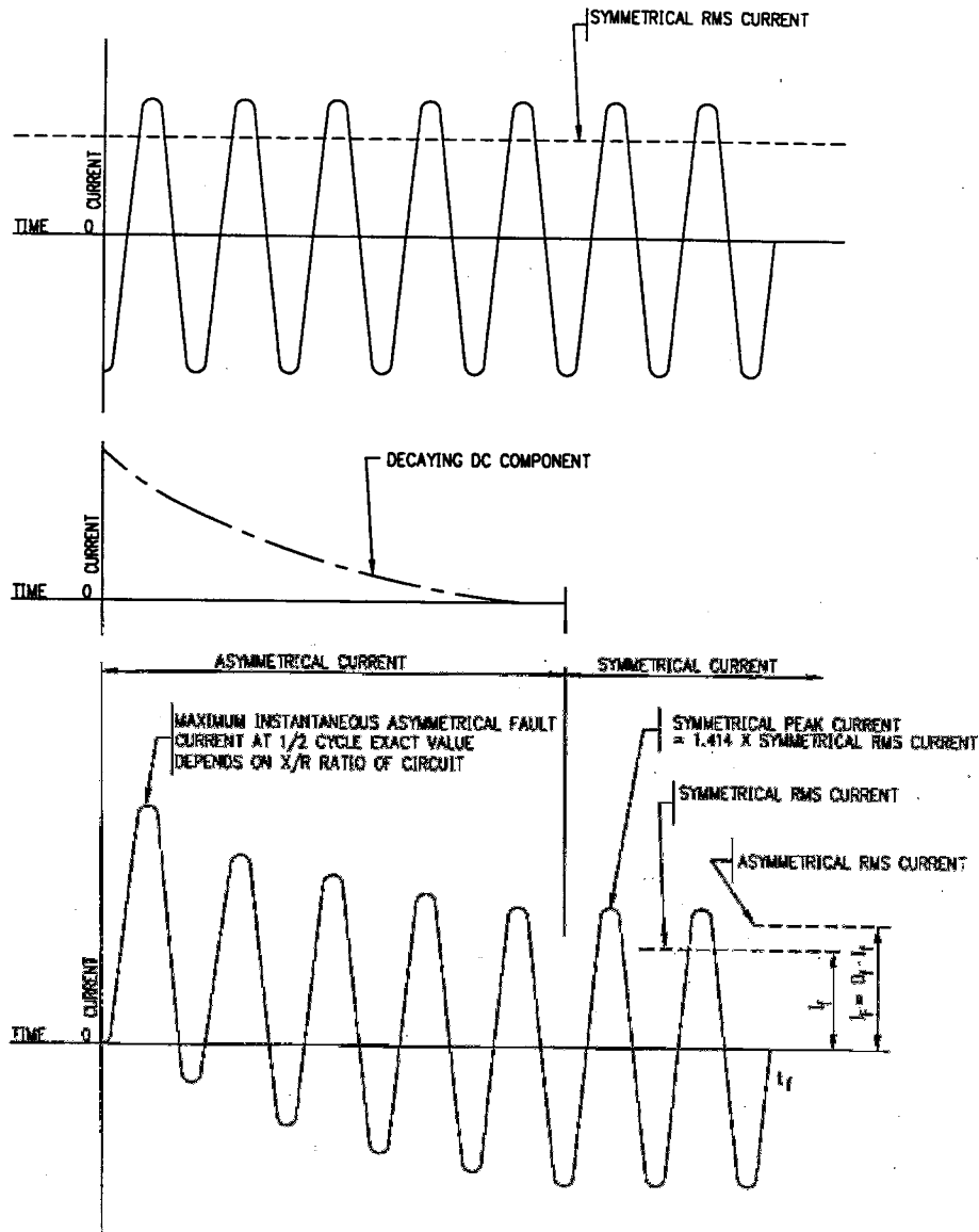
Figure 1—Relationship between actual values of fault current and values of I_f , I_r , and D_f for fault duration t_f
