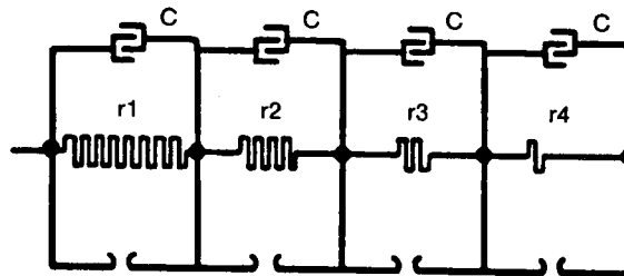
Figure 17—Soil model
