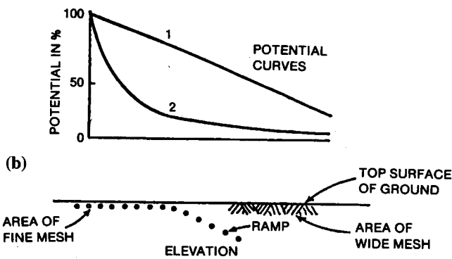
Figure G.9—Potential distribution in a ground mat with ramp (Curve 1) and without ramp (Curve 2)
