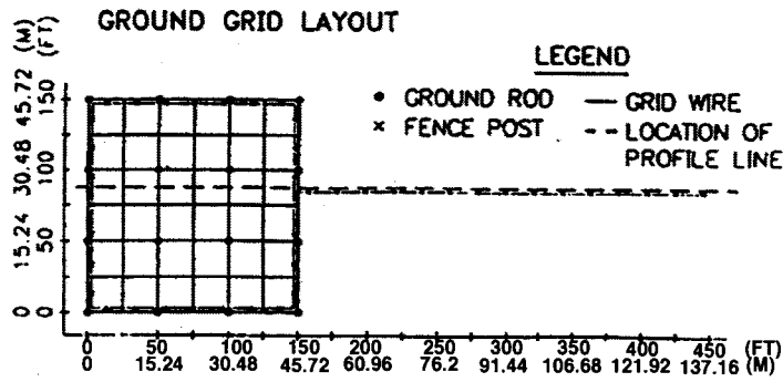
Figure 47—Transfer potential on a fence
