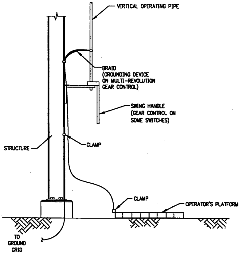
Figure 34—Typical switch shaft grounding
