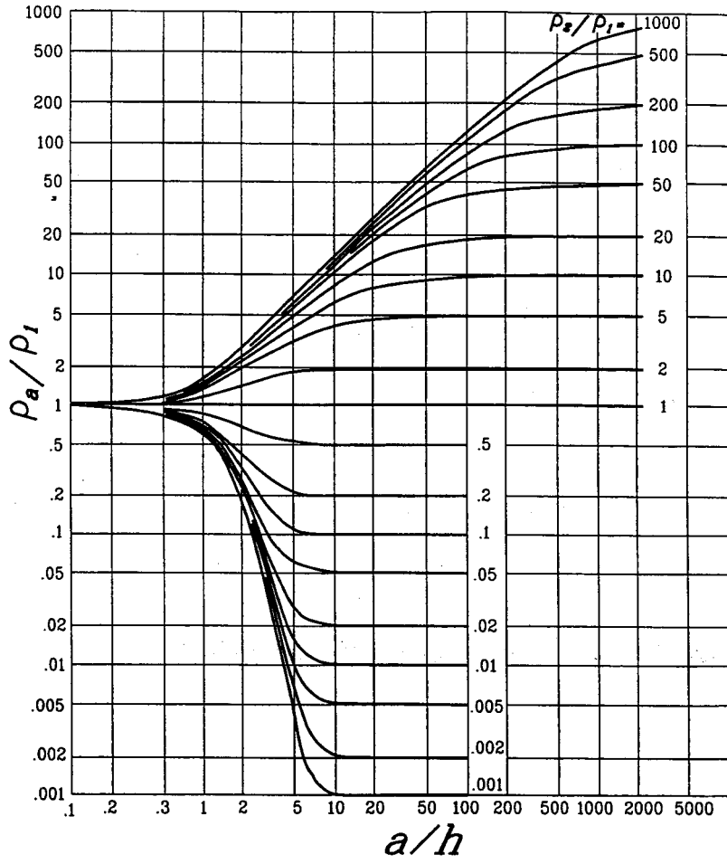
Figure 21—Sunde's graphical method
