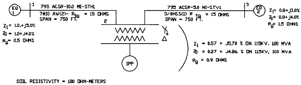
Figure C.23—System and configuration data for example 1 of C.3
