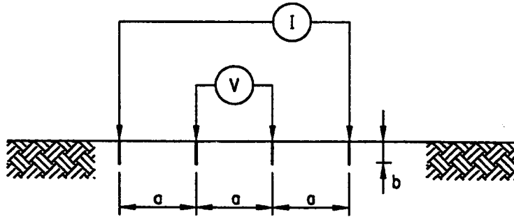
Figure 19—Wenner four-pin method
