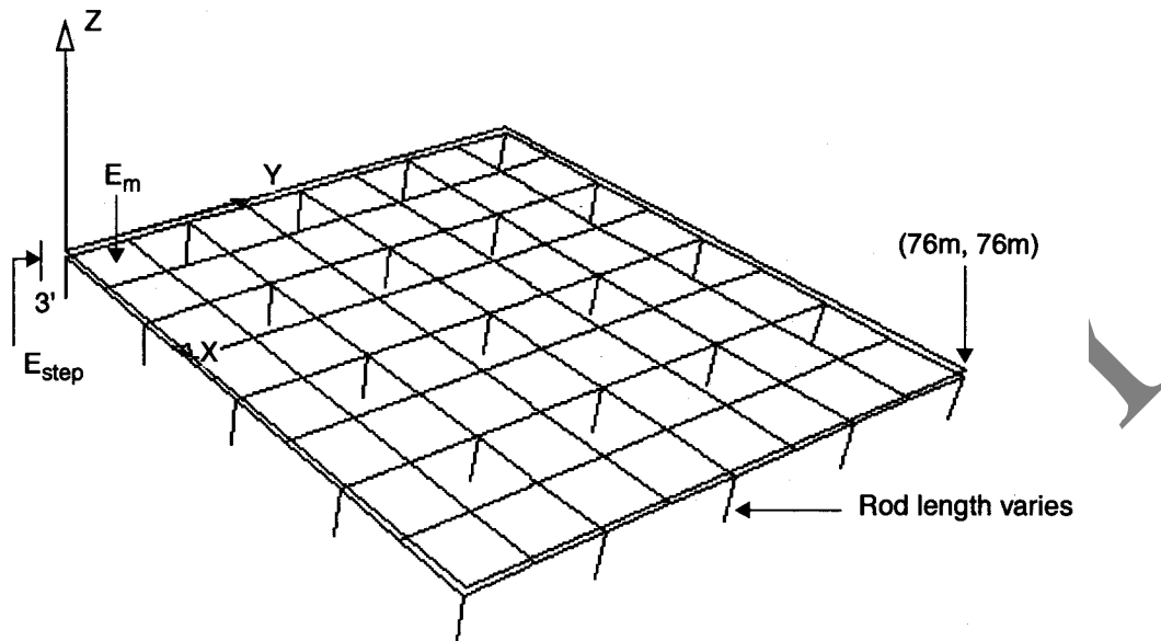
Figure E.1 – The ground grid modeled for computing grounding parameters
