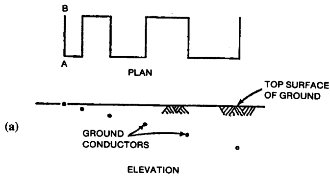
Figure G.8—Potential distribution for ground mats with fine meshes in portions
