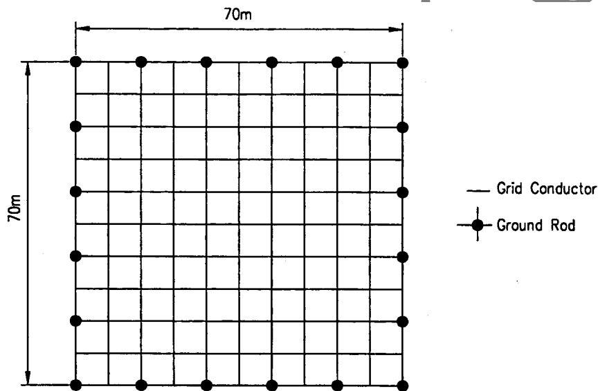
Figure B.2—Square grid with 20 7.5 m rods
