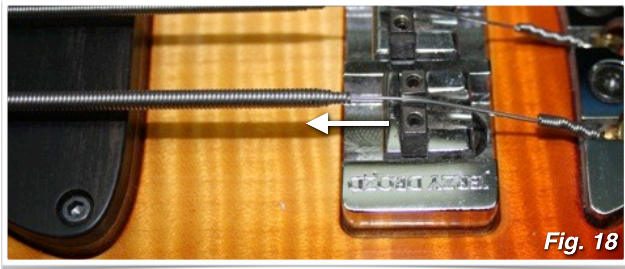
The lower the pitch at the 12 th fret in relation to the harmonic, the more you will have to move the saddle toward the pickups to shorten the string. Move the saddle toward the pickups if the note is lower than the harmonic.
