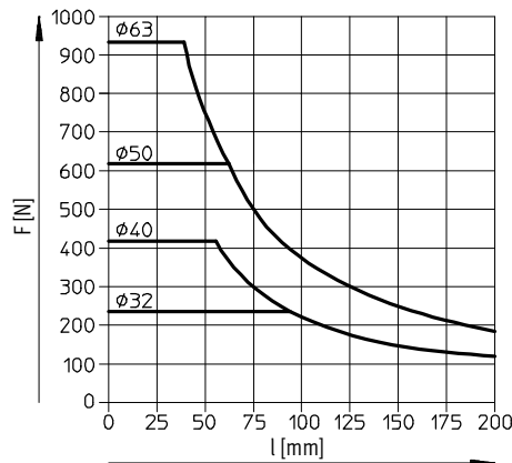
DFM-32 ... 63-GF Stroke 80 ... 100 mm
