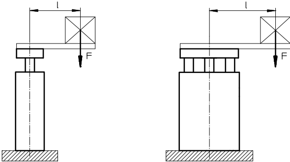
DFM-32 ... 63-KF Stroke 125 ... 200 mm
