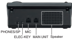
Controller Rear Panel View
