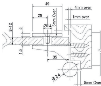
LAMP PH-01 (2 Way Adjustable Pivot Hinge)
