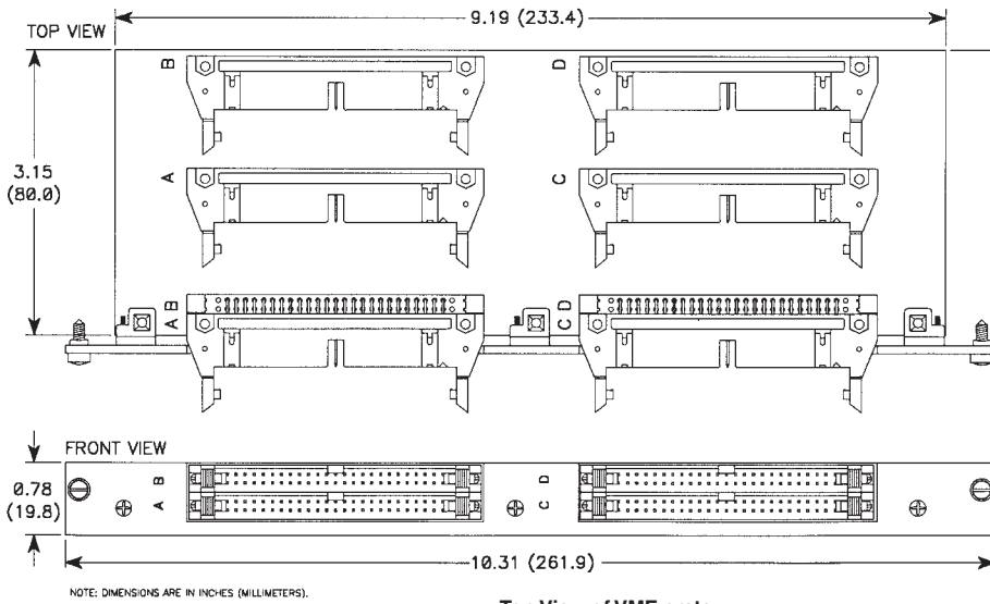
Top View of VME crate
