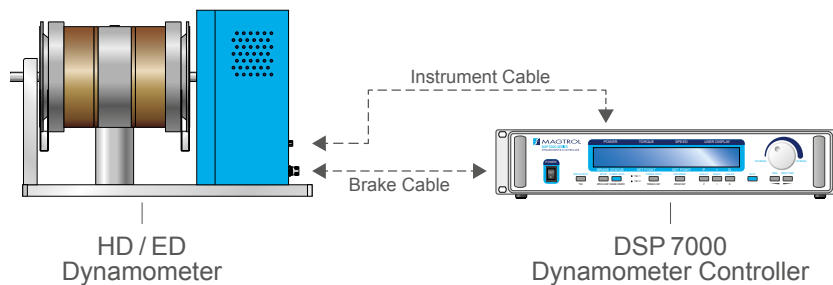
Fig. 2: Dynamometer with DSP 7000 Dynamometer Controller
