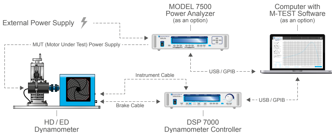
Fig. 3: Dynamometer with MODEL 7500 Power Analyzer, DSP7000 Dynamometer Controller and M-TEST Software
