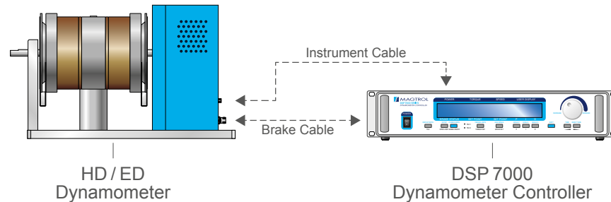
Fig. 2: Dynamometer with DSP7000 Dynamometer Controller
