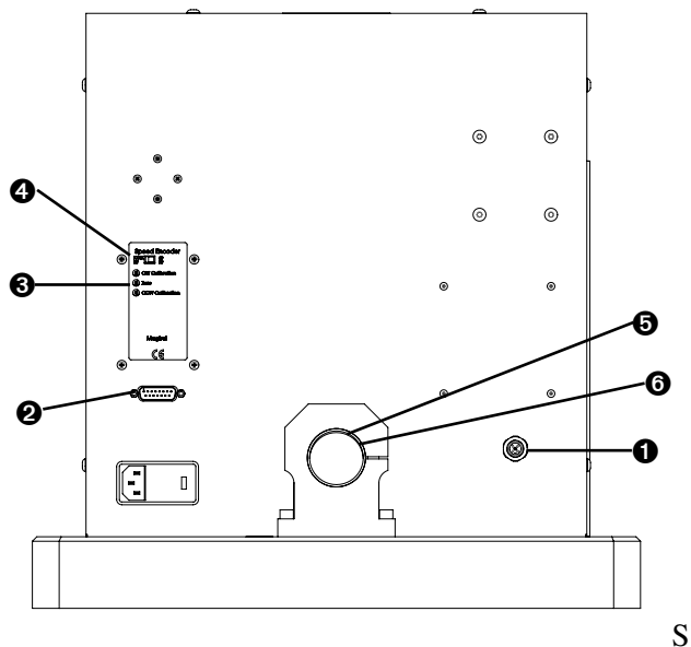
Figure 2-1 Rear Panel
