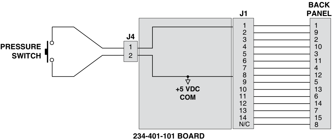
Figure 3–9 Air Flow Sensor Schematic
