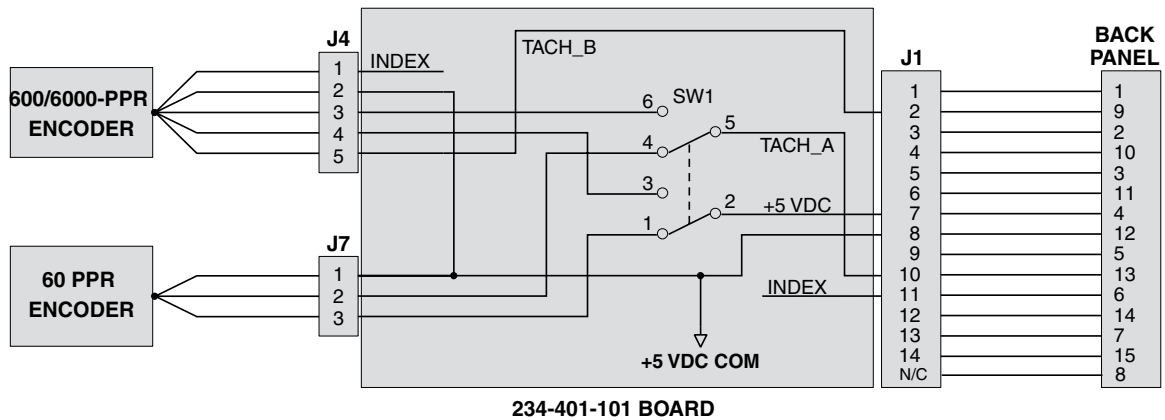
Figure 7-1 Speed Encoder Schematic
