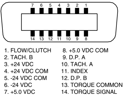
Figure 2–5 Prior to 2020 Dynamometer Connector
