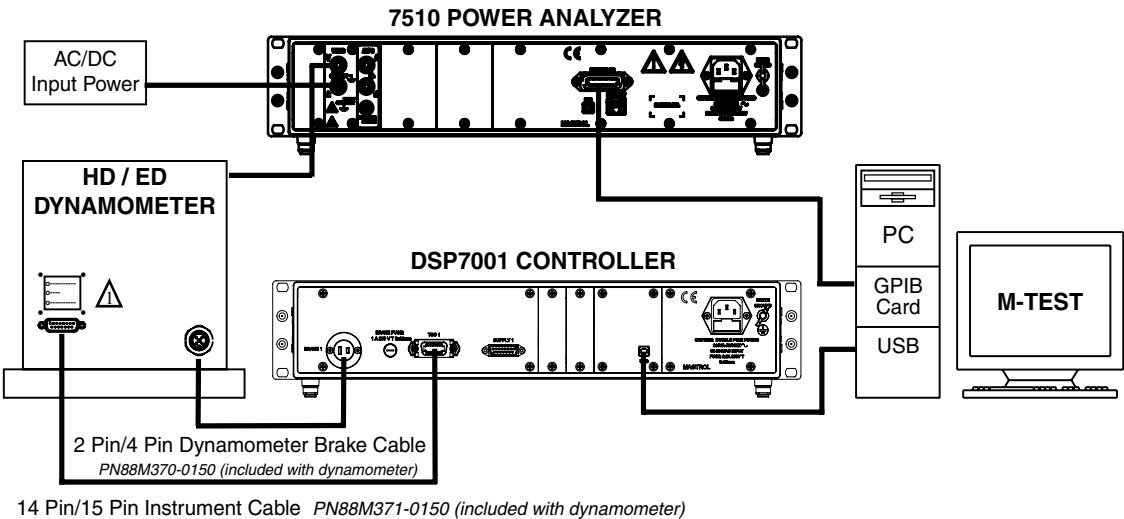
Figure 3–8 Dynamometer with 7510 Power Analyzer, DSP7001 Controller and M-TEST Software
