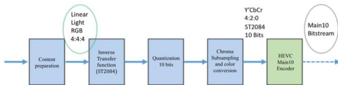
Figure 9: HDR10 content mastering process. Image credit: NGCodec
