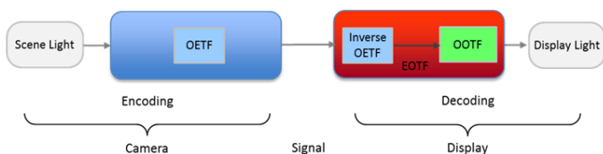
Figure 16: In an HLG system, the OETF (rendering intent) is applied in the display. Image credit: ITU
