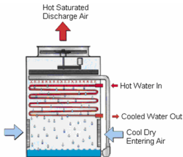
CLOSED CIRCUIT COOLER
