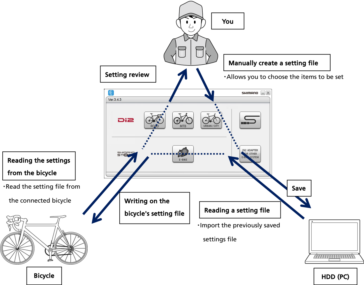
Flowchart
