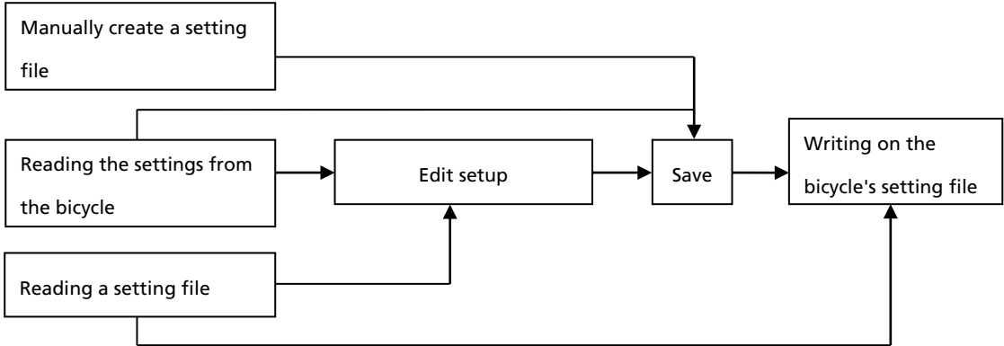
Flowchart
