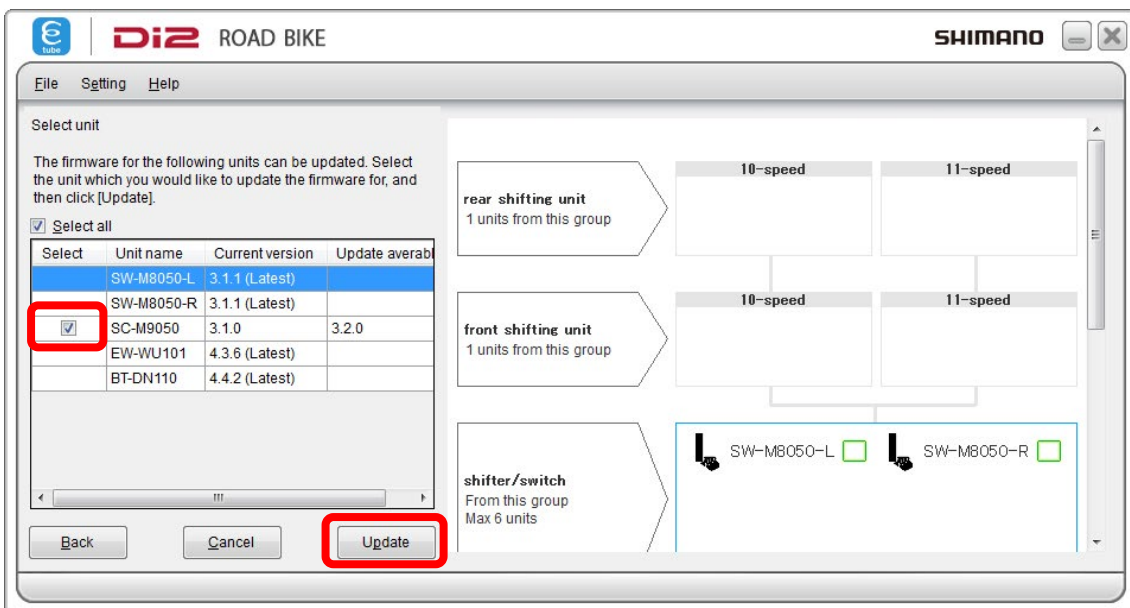
(Unit selection screen)
