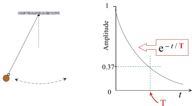
Figure 1.5 A pendulum serves as simple analogue (but not at all a direct model!) for proton resonance and T_1 relaxation. The oscillatory motion is affected by friction-like forces that cause it to fall off exponentially over time with a characteristic time 'T.' Analogous phenomena are responsible for the decline of a NMR signal at the rate 1/T_1 or 1/T_2 .
