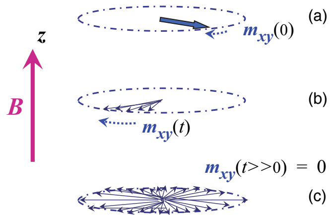
Figure 1.4 The ‘classical’ view is clearly incompatible with the ‘quasi-QM’. (a) The magnetization of a cohort of protons, \mathbf{m}_{xy}(t) , starts out precessing like a single, narrow vector in the plane transverse to \mathbf{B}_z . (b) Over time, the protons precess at slightly different rates because of minute differences in their local environments, and they begin to lose phase coherence. The transverse magnetization spreads out and diminishes at the rate 1/T_2 , as e^{-t/T_2} . (c) After a period several times the tissue’s transverse or spin-spin relaxation time , T_2 , the protons will be pointing every which way, the sum of their spin vectors will be zero, and \mathbf{m}_{xy}(t \gg T_2) will vanish.
