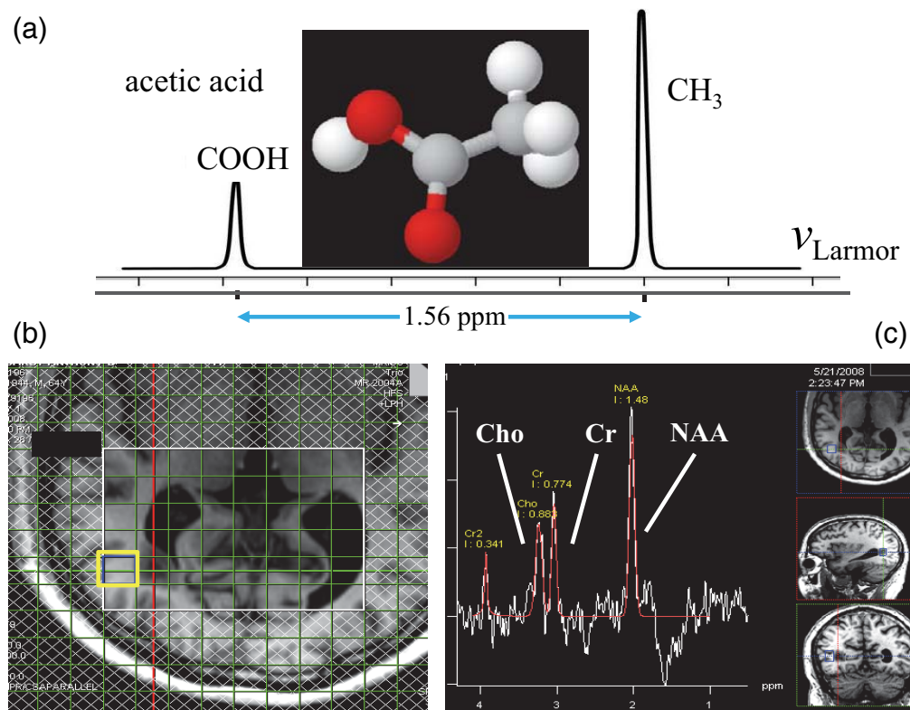
Figure 1.7 An MRS spectrum (a) reflects the uneven circulation of electrons within a molecule (acetic acid) that give rise to small variations in local magnetic field, hence in parts per million (ppm) chemical shifts in proton Larmor frequency. (b) Tissue just outside the patient's lesion (yellow box) yields a normal MRS spectrum. The spectrum from the lesion itself appears nearly identical, (c) but its higher Cr/NAA and Cho/NAA ratios are characteristic of a glioma.
