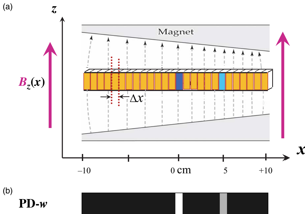
Figure 1.3 This 1D phantom consists of a row of small, hollow chambers, all of width \Delta x . (a) The one at x = 0 cm contains twice as much water as that at 5 cm, and the others are empty. The main magnetic field points upward along the z -axis at each chamber, but the x -gradient component causes the strength of the net local field at each voxel, B_z(x) , to increase linearly with position x . Field strength increases as the dashed field lines come closer together. Each of the two water samples undergoes NMR at a different, but precisely measurable frequency. This is an encoding technique that allows determination of voxel position along the x -axis (b), which makes possible the creation of a MR image of proton density (PD) along the phantom. The greater the PD in a voxel, the brighter the pixel shines on the display.
