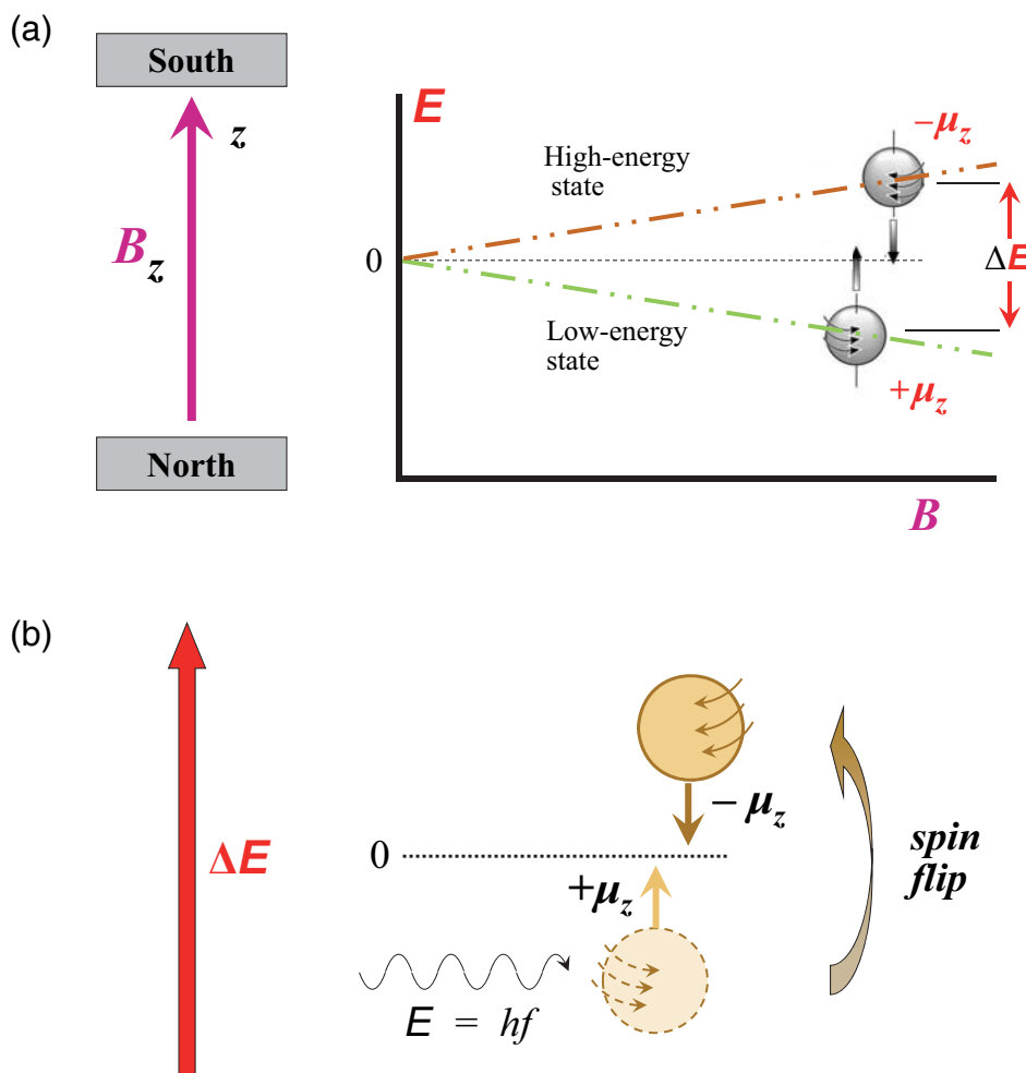
Figure 1.2 There are two pedagogical pictures of NMR, the quasi-QM and the classical , that are commonly drawn upon in introducing MRI physics. The two are mutually incompatible and inconsistent, and they cannot be combined together, because of the quite different assumptions adopted in constructing each of them out of the fully correct, rigorous quantum theory. But both are useful in different ways. Here we discuss only the greatly simplified quasi-QM picture. (a) A single proton behaves like a tiny compass needle, but it can align in an externally magnetic field, B_z , only along or against it and the z-axis. The energy levels for the two quasi-QM proton spin states diverge by the amount of the Zeeman energy, which is linear in the strength of the total local magnetic field. Nearly all of this B_z comes from the main magnet, and is constant. Much of the rest is from the intermittently activated gradient coils , and from the brief pulses from the RF (radiofrequency) transmitter . Finally, the amount of random RF ‘noise’ generated by fluctuations in molecular motions is tiny, but it greatly influences proton spin relaxation processes. A spin- 1/2 nucleus such as a proton is allowed to inhabit either one of the two levels: in the lower-energy, ‘spin-up’ state, the projection of \mu onto the z-axis is aligned parallel to B_z . Alternatively, in the ‘down,’ high-energy state, it points against B_z . Also, unlike a compass needle, a proton can remain for long periods of time in a quasi-stable, higher-energy spin-orientation state, pointing the ‘wrong’ direction. (b) The two spin states differ by the Zeeman energy, \Delta E = 2\mu_z B_z . A photon (or phonon) of the right energy can cause a transition up or down between the two. The horizontal dashed line in the middle indicates the energy the nucleus has at B_z = 0 .
