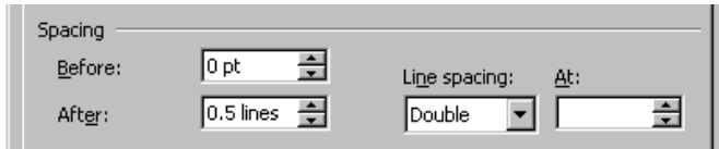
Fig 14.2 Heuristic rules
