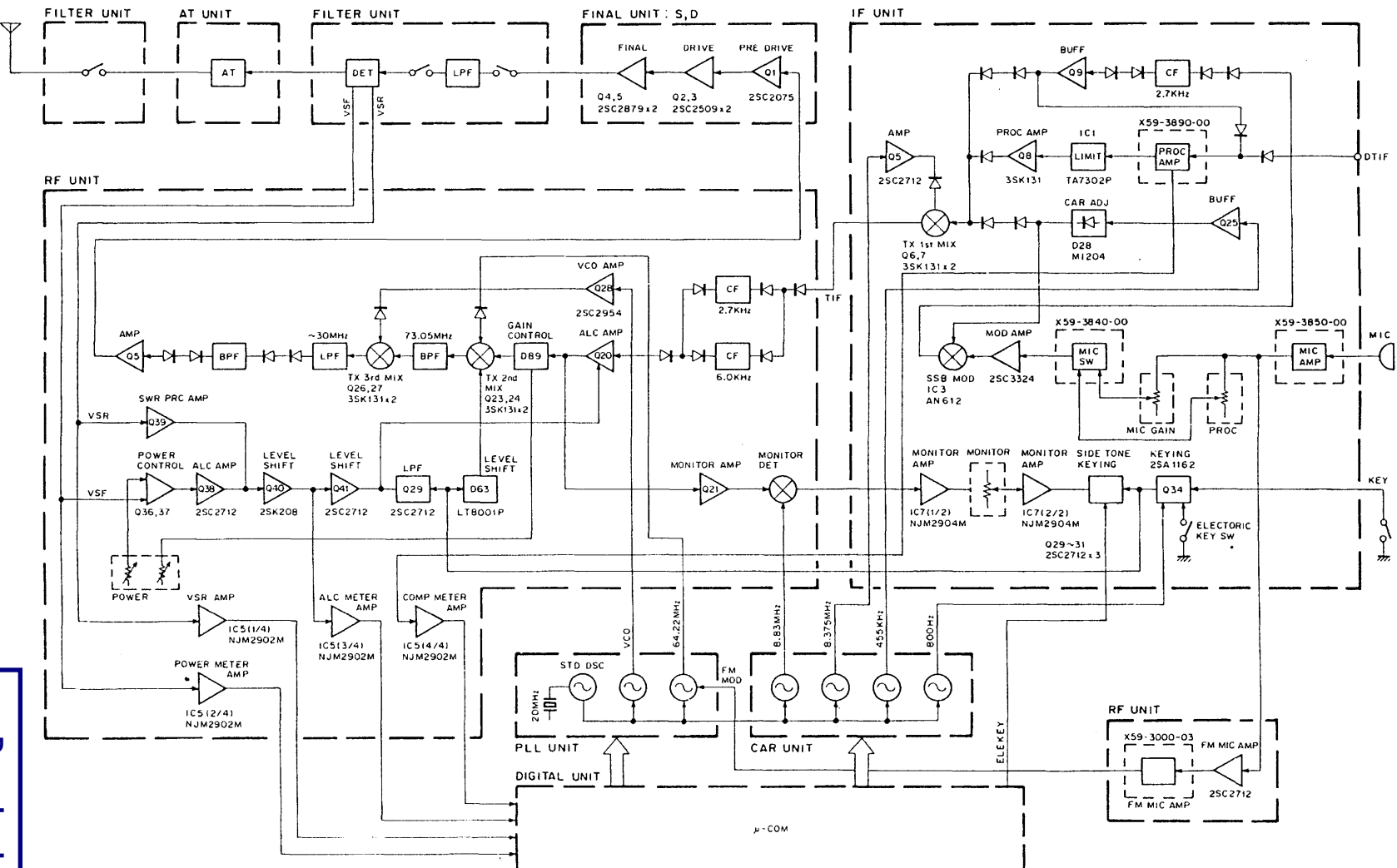
Fig. 8 Transmitter circuit block diagram
