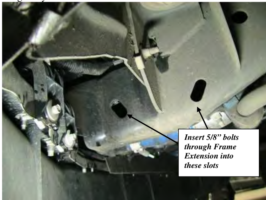
Figure 13: LH frame rail
