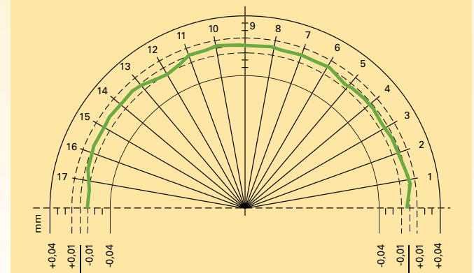
GF 500 radius tolerance ( \pm 0.01 mm, \pm 0.0004'' )
