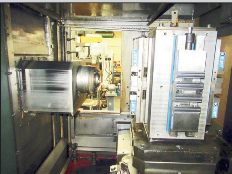
ENSHU CNC HORIZONTAL MACHINING CENTER (INSIDE VIEW)
