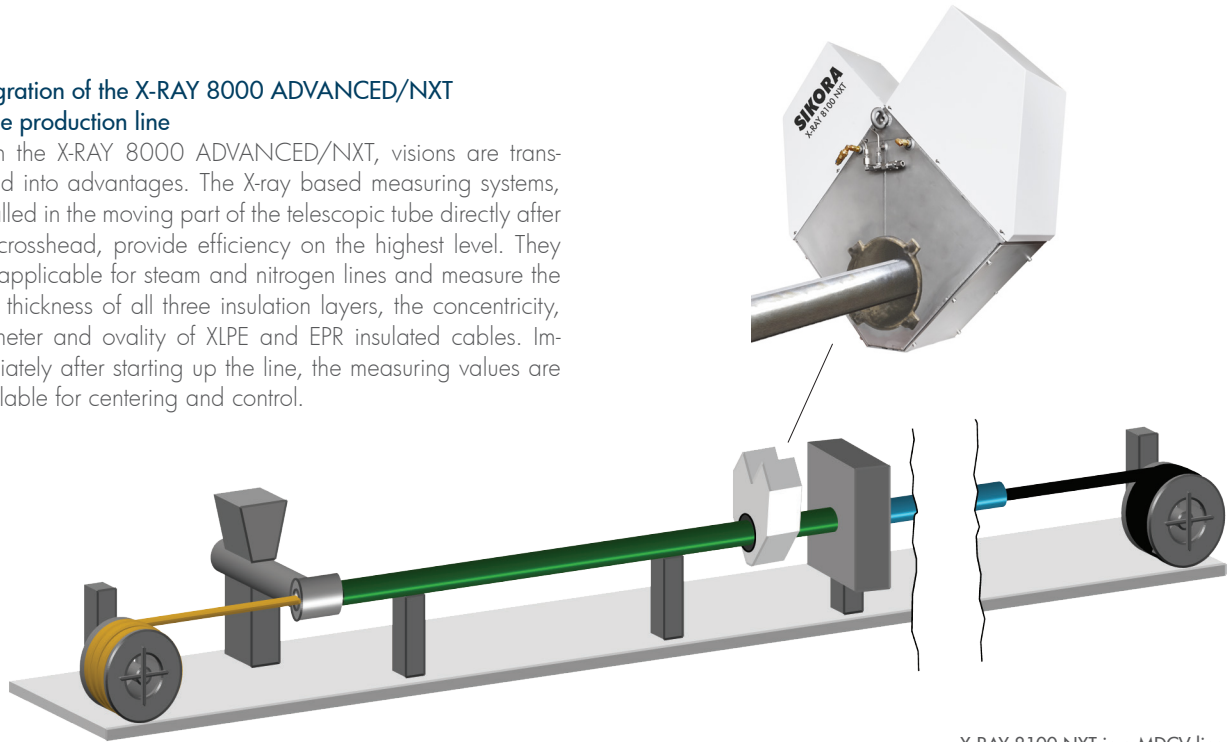
X-RAY 8100 NXT in a MDCV line
