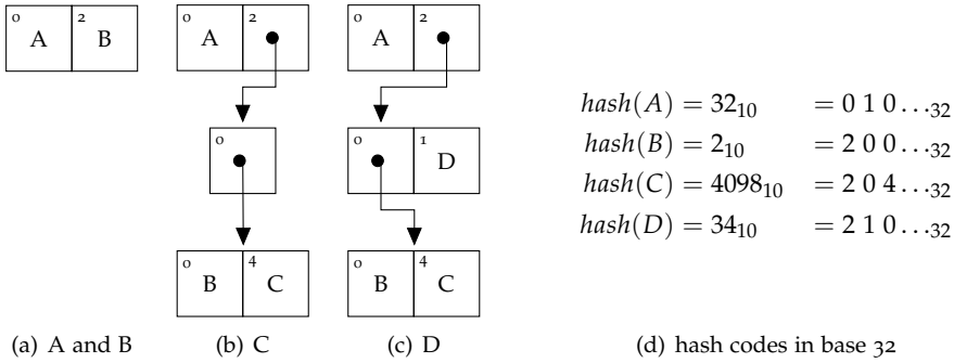
Figure 3.1: Inserting three integers into a HAMT-based set (3.1(a), 3.1(b), and 3.1(c)), on basis of their hashes (3.1(d)).
