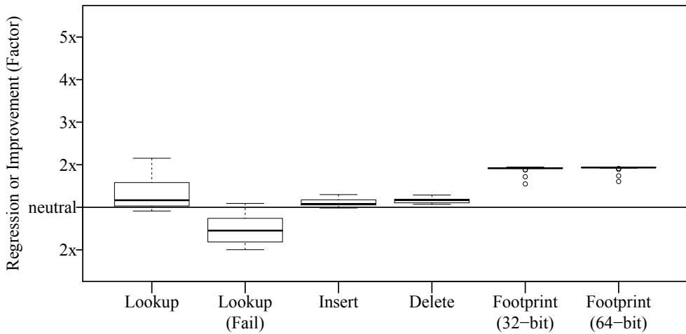
(b) Specialized HHAMT multi-map versus Scala's multi-map (baseline).
