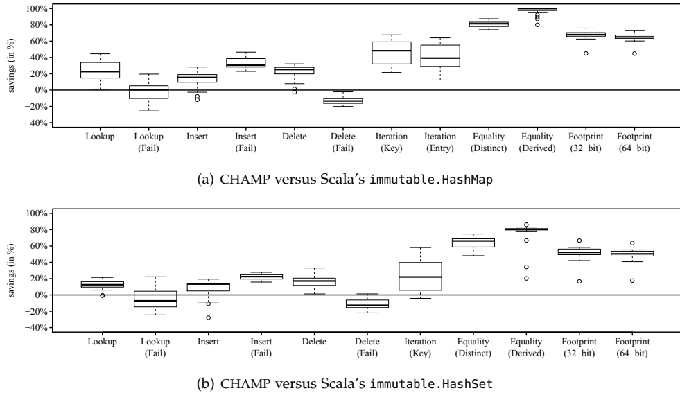
Figure 3.6: Runtime and memory savings of CHAMP compared to Scala's immutable.HashMap , Set .
