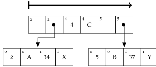
(a) Current HAMT ordering with 1-bit state.
