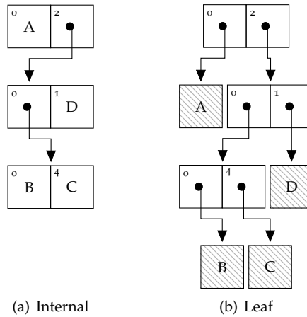
Figure 3.3: HAMT-based sets with values in internal nodes versus values at the leaves.
