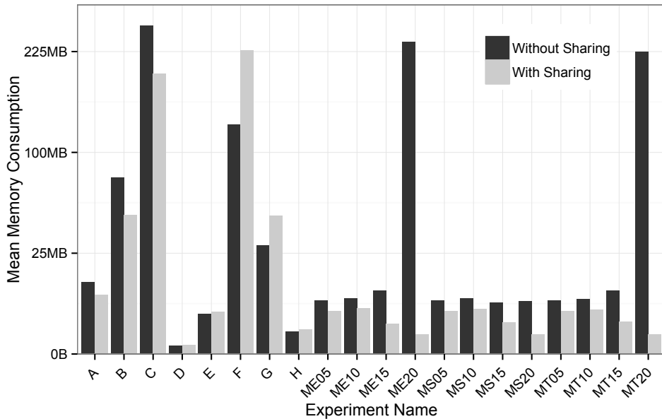
Figure 6.7: Effect of Maximal Sharing on Memory Consumption
