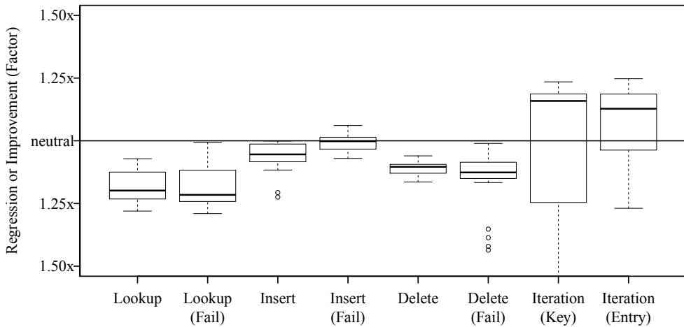
(b) HHAMT multi-map versus CHAMP map (baseline).
