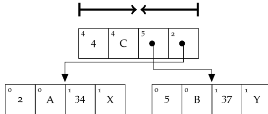
(c) Final CHAMP ordering with 2-bit state.
