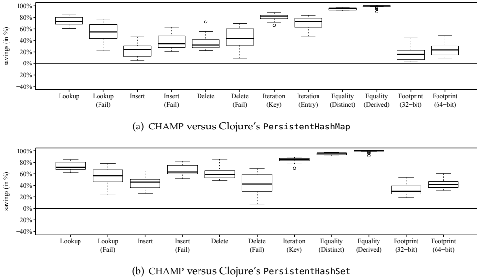
Figure 3.5: Runtime and memory savings of CHAMP compared to Clojure's PersistentHash{Map,Set}.
