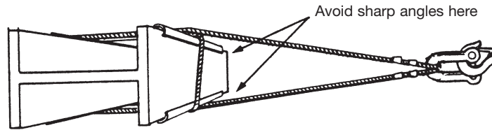
LASHING AROUND COLUMN OR BEAM Figure 7
