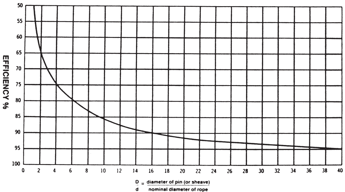
STRENGTH EFFICIENCY OF WIRE ROPE WHEN BENT OVER PINS OR SHEAVES OF VARIOUS SIZES Figure 8
