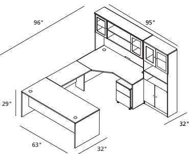
Combination 100-12-7 1/63/32 Desk 1/63/32/24L Crescent Desk 1/32/20 Return 1/19/20/3 Mobile Pedestal H/63/43 Hutch B/32/72 Bookcase A/183 Glass Doors (2 Sets) A/180 Wood Doors 1/155 Panel
