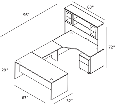
Combination 100-11-7 1/63/32 Desk 1/63/32/24L Crescent Desk 1/32/20 Return 1/19/20/3 Mobile Pedestal H/63/43 Hutch A/183 Glass Doors 1/155 Panel
