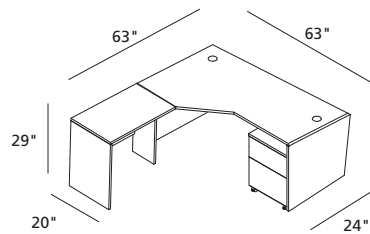
Combination 100-14-7 1/63/32/24L Crescent Desk 1/32/20 Return 1/19/20/3 Mobile Pedestal
