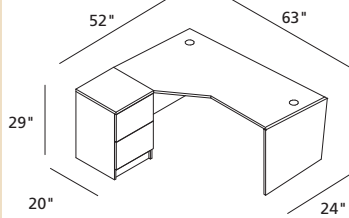
Combination 100-13-7 1/63/32/24L Crescent Desk 1/19/20/2 Two Drawer File
