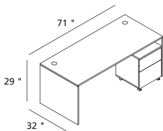
Combination 100-3-7 1/71/32 Desk 1/19/20/3 Mobile Pedestal
