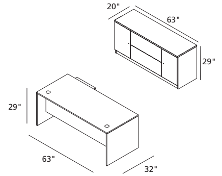
Combination 100-7-7 1/63/32 Desk 1/19/20/3 Mobile Pedestal 1/63/20/2 Credenza
