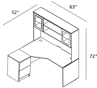
Combination 100-16-7 1/63/32/24L Crescent Desk 1/19/20/2 Two Drawer File H/63/43 Hutch A/183 Glass Doors
