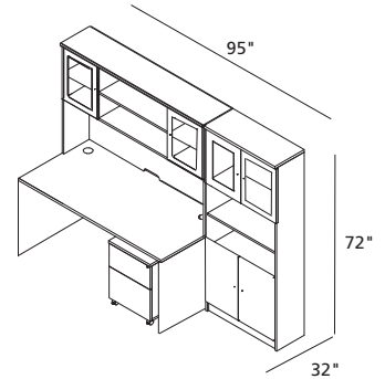
Combination 100-21-7 1/63/32 Desk 1/19/20/3 Mobile Pedestal H/63/43 Hutch B/32/72 Bookcase A/183 Glass Doors (2 Sets) A/180 Wood Doors
