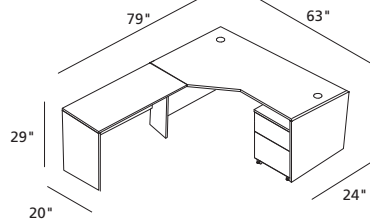
Combination 100-15-7 1/63/32/24L Crescent Desk 1/47/20 Return 1/19/20/3 Mobile Pedestal
