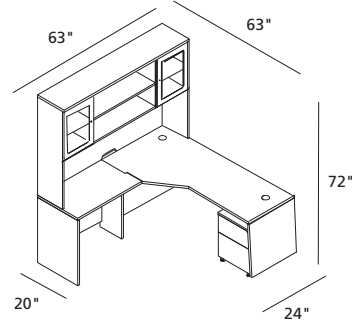
Combination 100-17-7 1/63/32/24L Crescent Desk 1/32/20 Return 1/19/20/3 Mobile Pedestal H/63/43 Hutch A/183 Glass Doors
