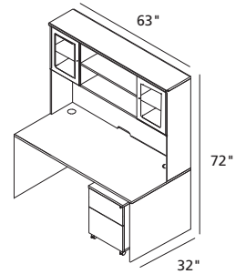
Combination 100-20-7 1/63/32 Desk 1/19/20/3 Mobile Pedestal H/63/43 Hutch A/183 Glass Doors
