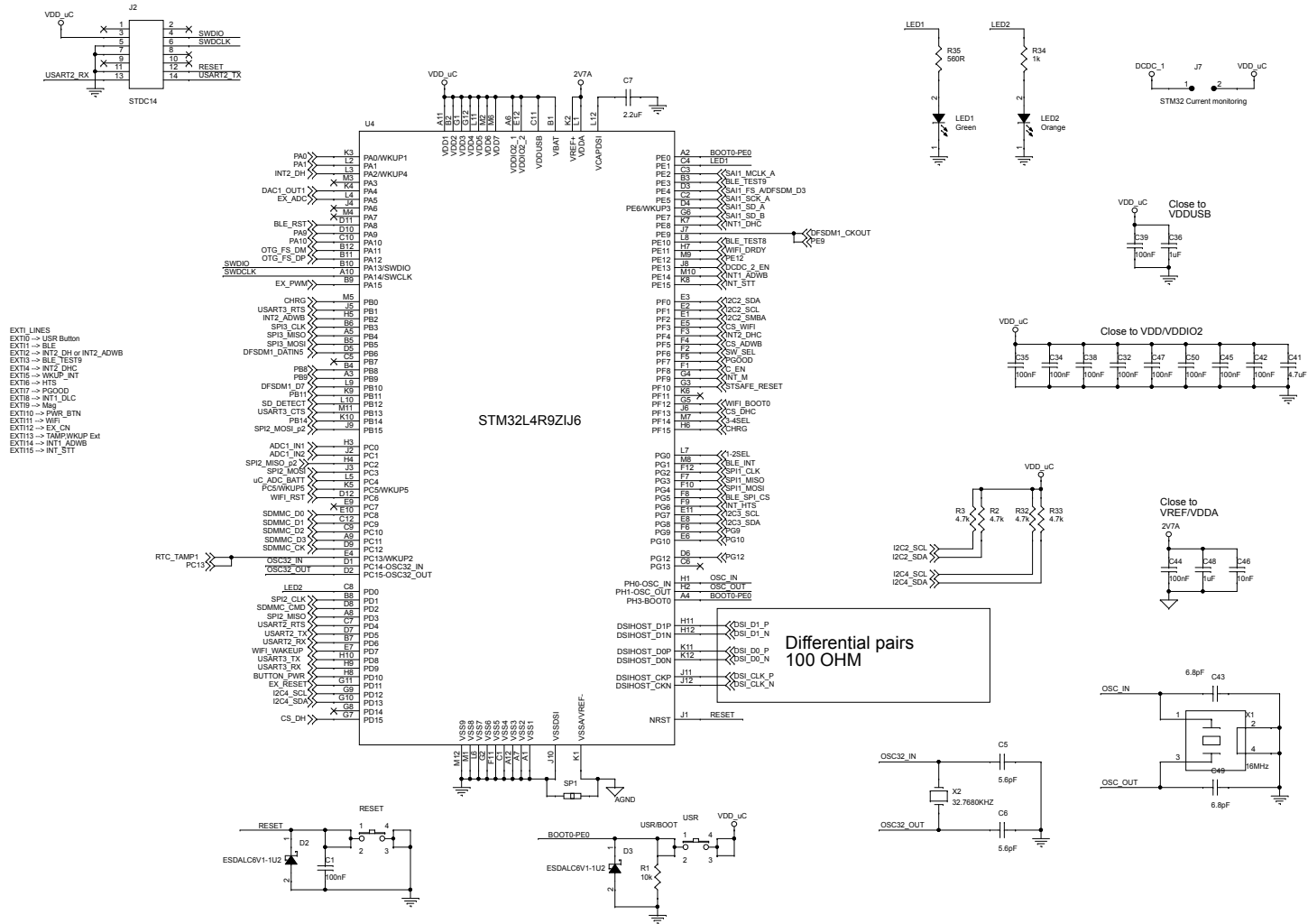
Figure 34. STEVAL-STWINKT1 schematic - MCU
