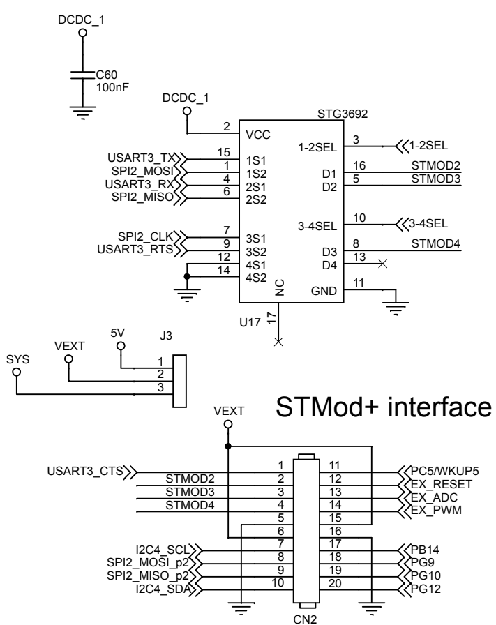
Figure 32. STEVAL-STWINKT1 schematic - connectors
