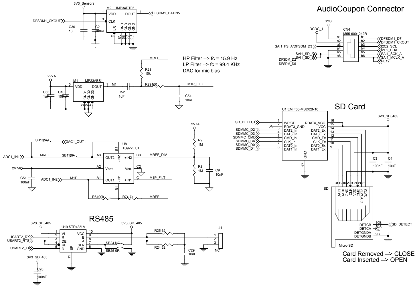
Figure 35. STEVAL-STWINKT1 schematic - audio, RS485, SD card
