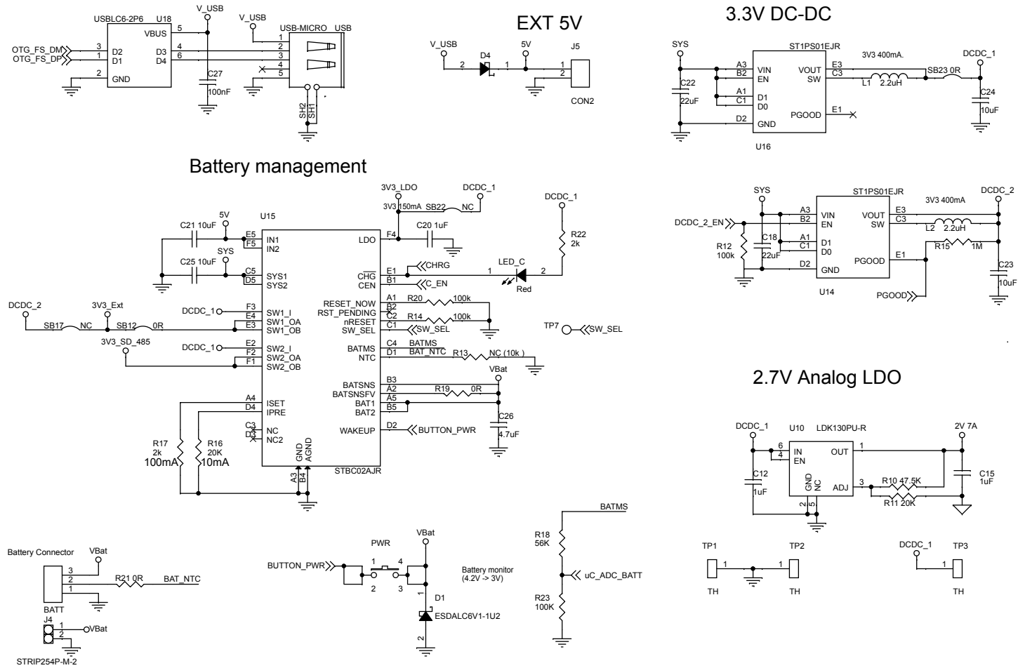
Figure 31. STEVAL-STWINK1 schematic - power
