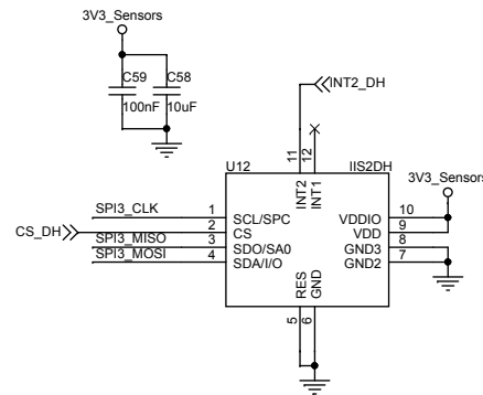
Accelerometer
