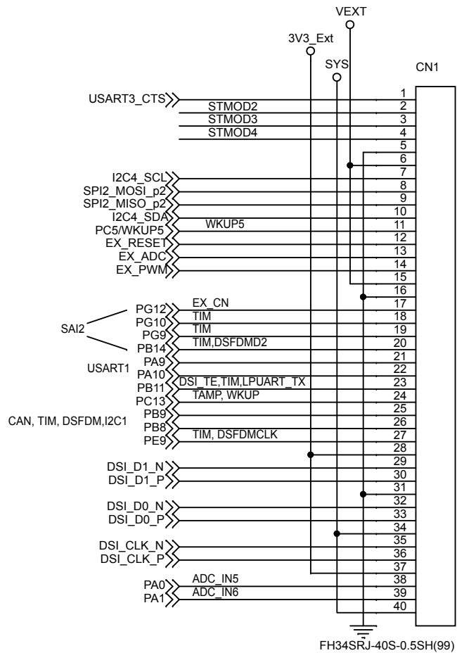
Figure 32. STEVAL-STWINKT1 schematic - connectors
