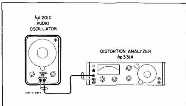
Figure 5-3. Distortion Check
