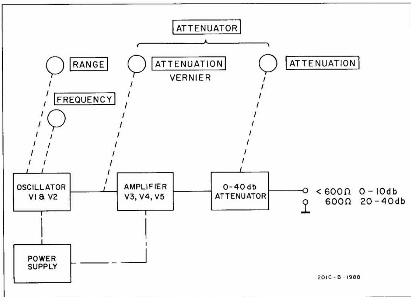
Figure 4-1. Block Diagram of Model 201C
