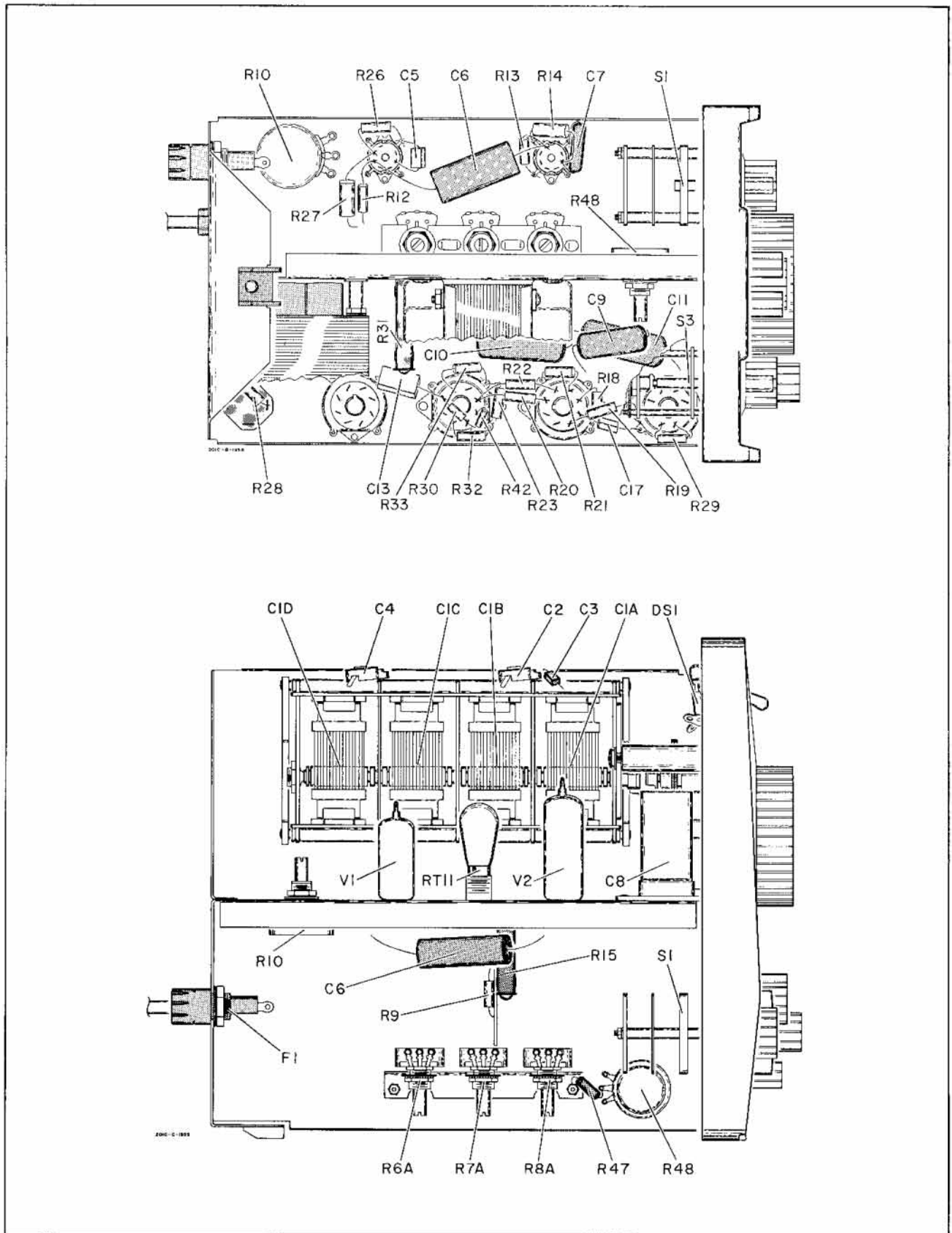
Figure 5-5. Bottom and Right Side Views
