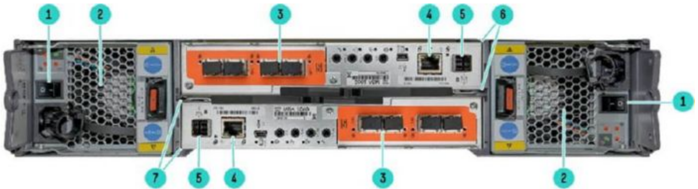
HPE MSA 2060 Storage
