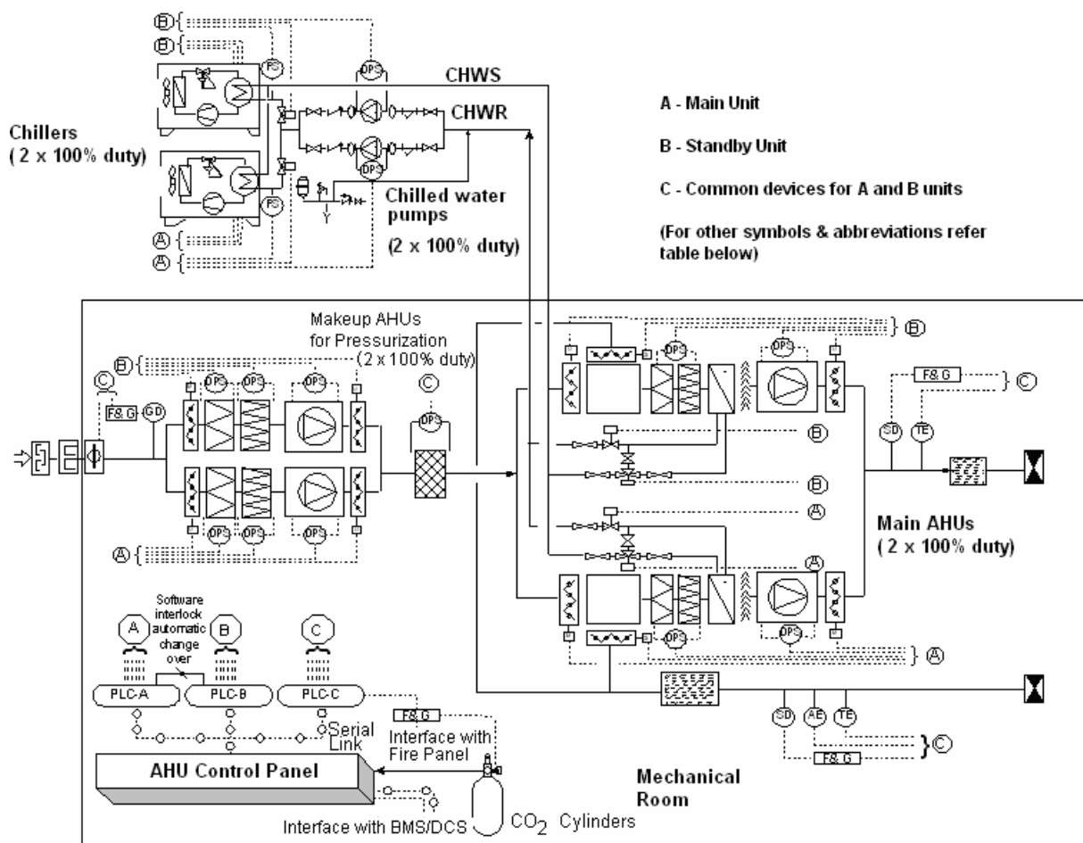
TYPICAL CONTROL DIAGRAM FOR OIL &amp; GAS FACILITY
