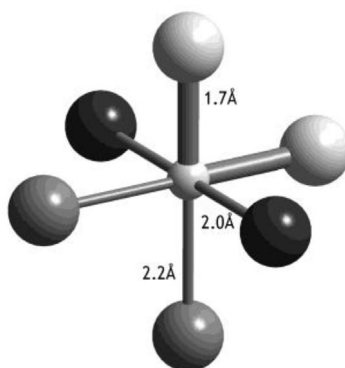
Fig. 9 Structure of \text{VO}_2(\text{H}_2\text{O})_4^+ in aqueous solution, ref. [12].
