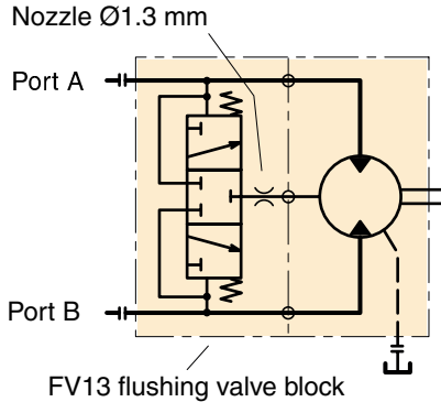
Hydraulic schematic.
