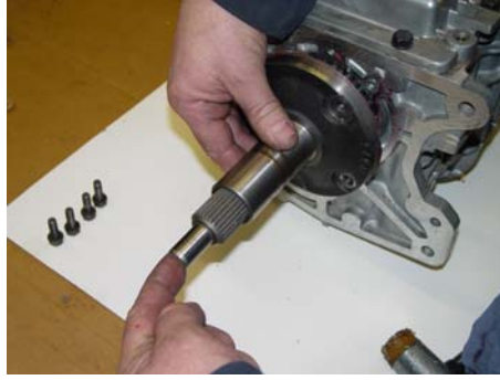
FIG. B REMOVE OLD RETAINER
