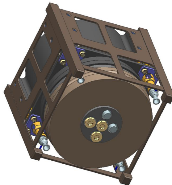
Figure 3: The CHAMPS integrates into a standard 1U frame
