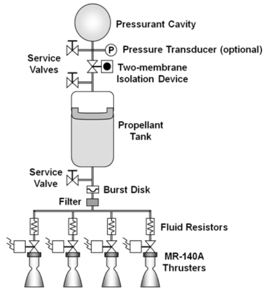
Figure 5: CHAMPS Functional Schematic
