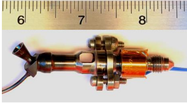
Figure 6: Aerojet MR-140 Thruster
