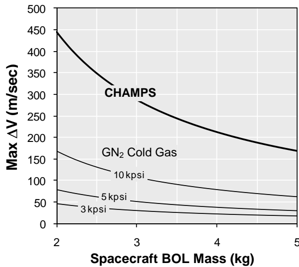
Figure 7: Comparison of maximum deliverable \Delta V for CHAMPS and 3, 5, and 10 kpsi 1U GN 2 cold gas systems
