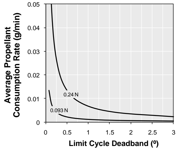
Figure 8: Estimated CHAMPS limit cycle propellant consumption rate at minimum BOL and EOL thrust
