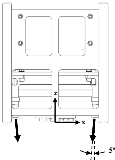
Figure 4: CHAMPS Thrust Vectors
