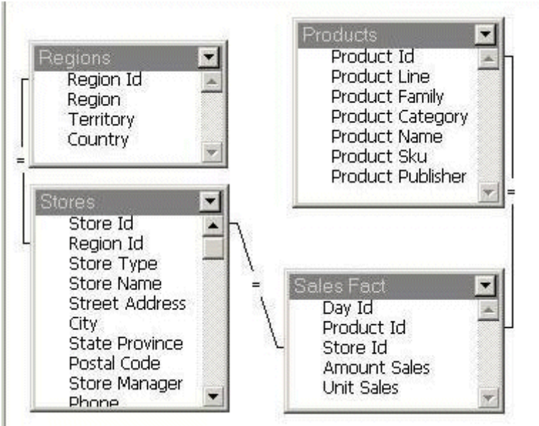
Figure 6 Database Layout Showing Possible Joins
